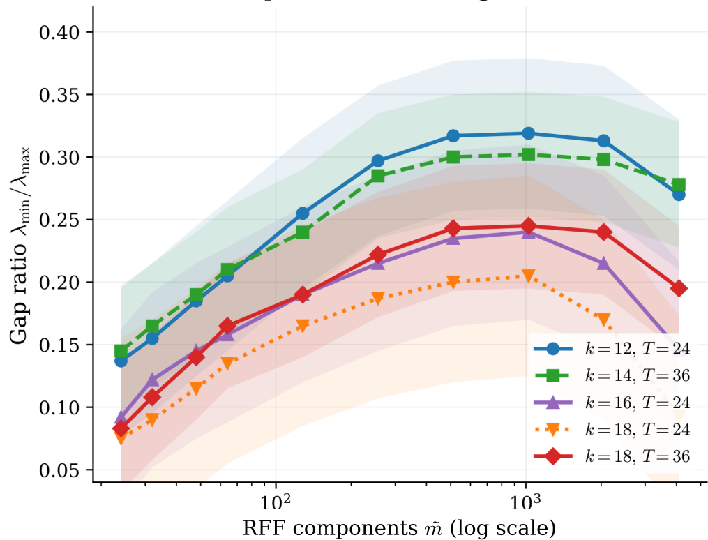
Gap ratio vs. RFF (log scale)
