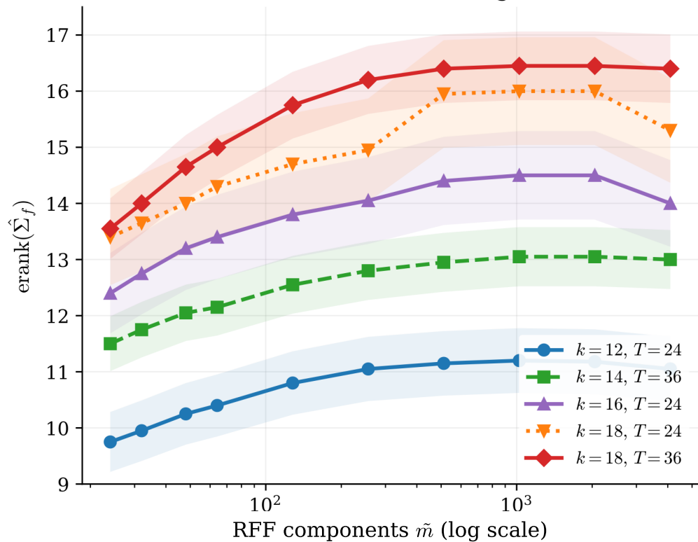
Effective rank vs. RFF (log scale)
