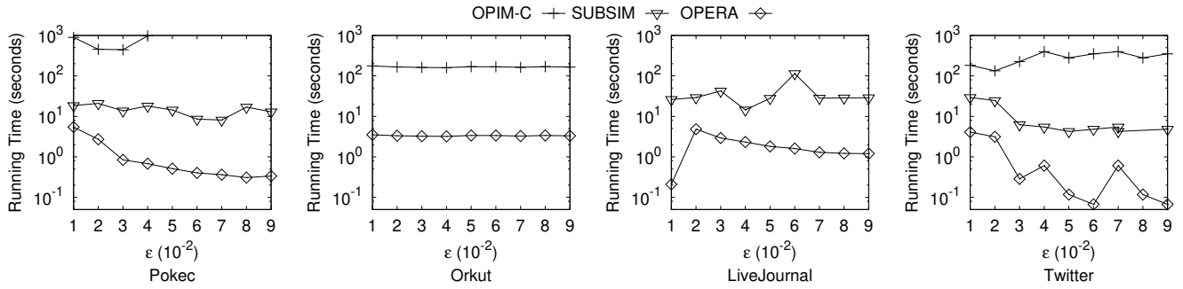
Figure 15: Effect of \epsilon on Running Time of All Algorithms under IC Model (Uniform Distribution)
