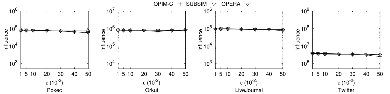
Figure 12: Effect of \epsilon on Influence of All Algorithms under IC Model (WC)
