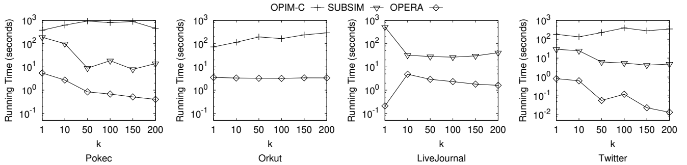
Figure 9: Effect of k on Running Time of All Algorithms under IC Model (Uniform Distribution)
