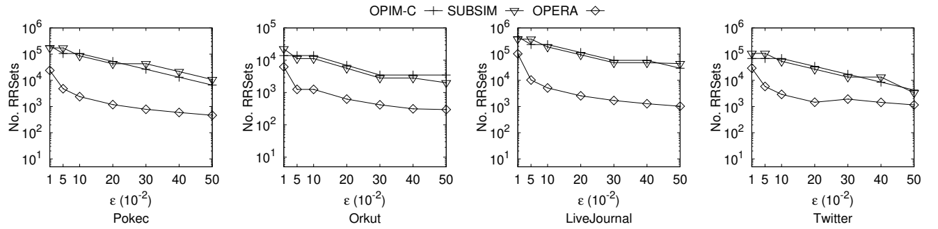
Figure 11: Effect of \epsilon on No. RR sets of All Algorithms under IC Model (WC)
