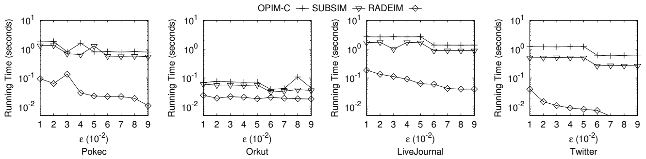
Figure 14: Effect of \epsilon on Running Time of All Algorithms under IC Model (Weibull Distribution)
