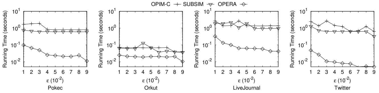
Figure 13: Effect of \epsilon on Running Time of All Algorithms under IC Model (Exponential Distribution)
