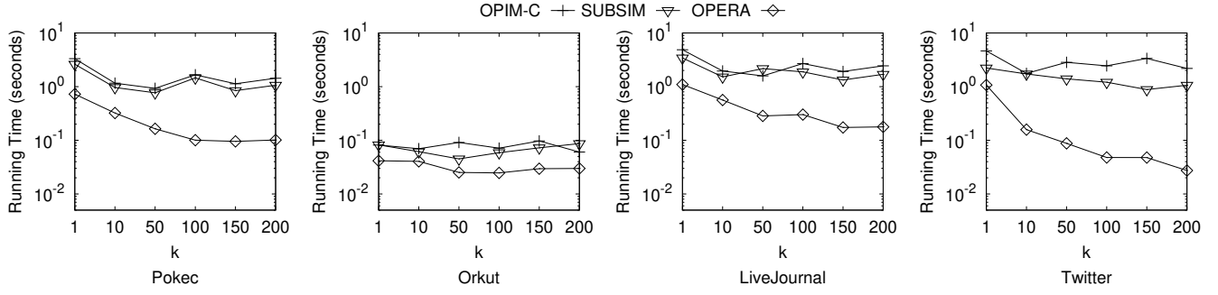
Figure 7: Effect of k on Running Time of All Algorithms under IC Model (Exponential Distribution)
