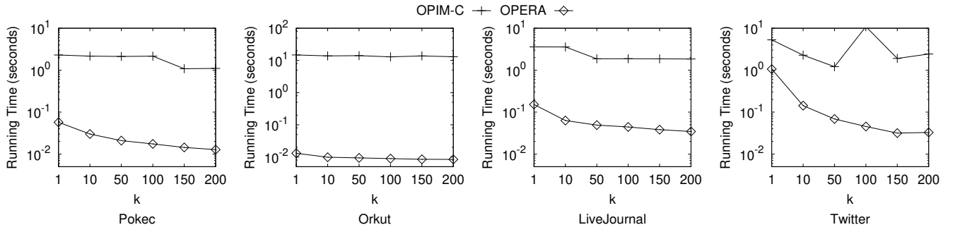
Figure 10: Effect of k on Running Time of All Algorithms under LT Model
