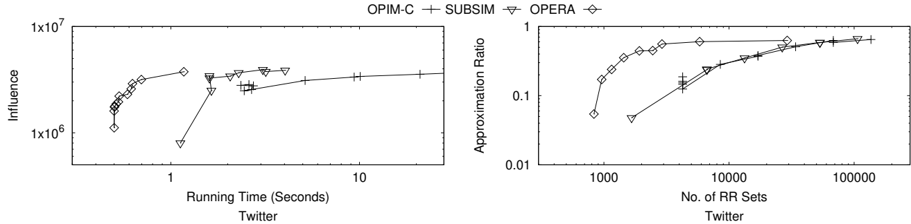
Figure 6: Influence Spread VS Running Time &amp; Appr. Ratio VS No. of RR Sets
