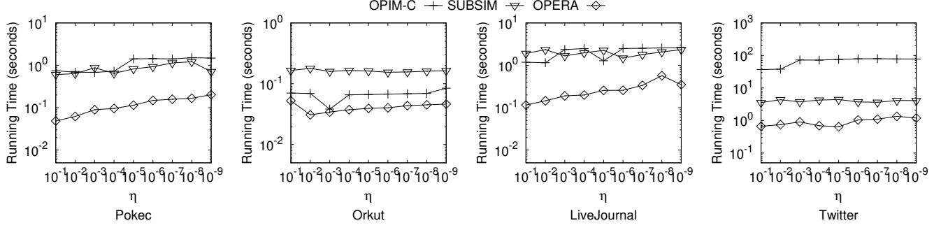
Figure 16: Effect of \eta on Running Time of All Algorithms under IC Model (WC)
