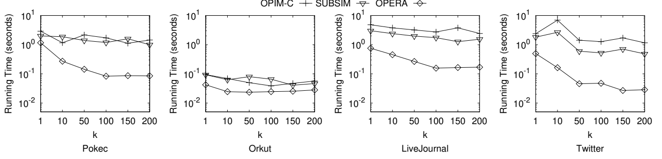
Figure 5: Effect of k on Running Time of All Algorithms under IC Model (Weibull Distribution)
