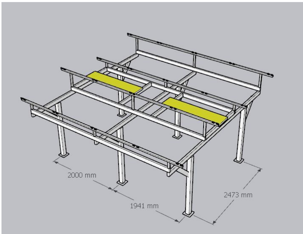
Structure details (5)
