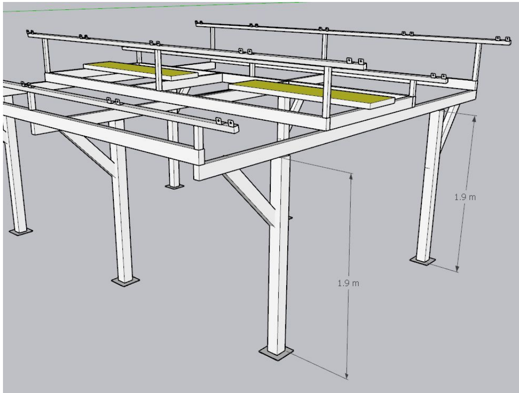
Structure details (2)
