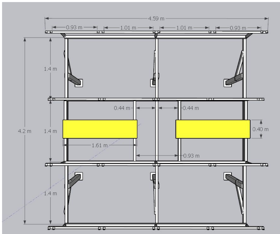
Structure details (1)
