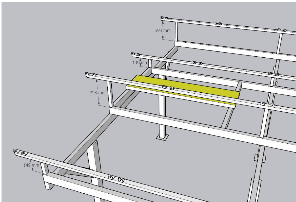
Structure details (7)
