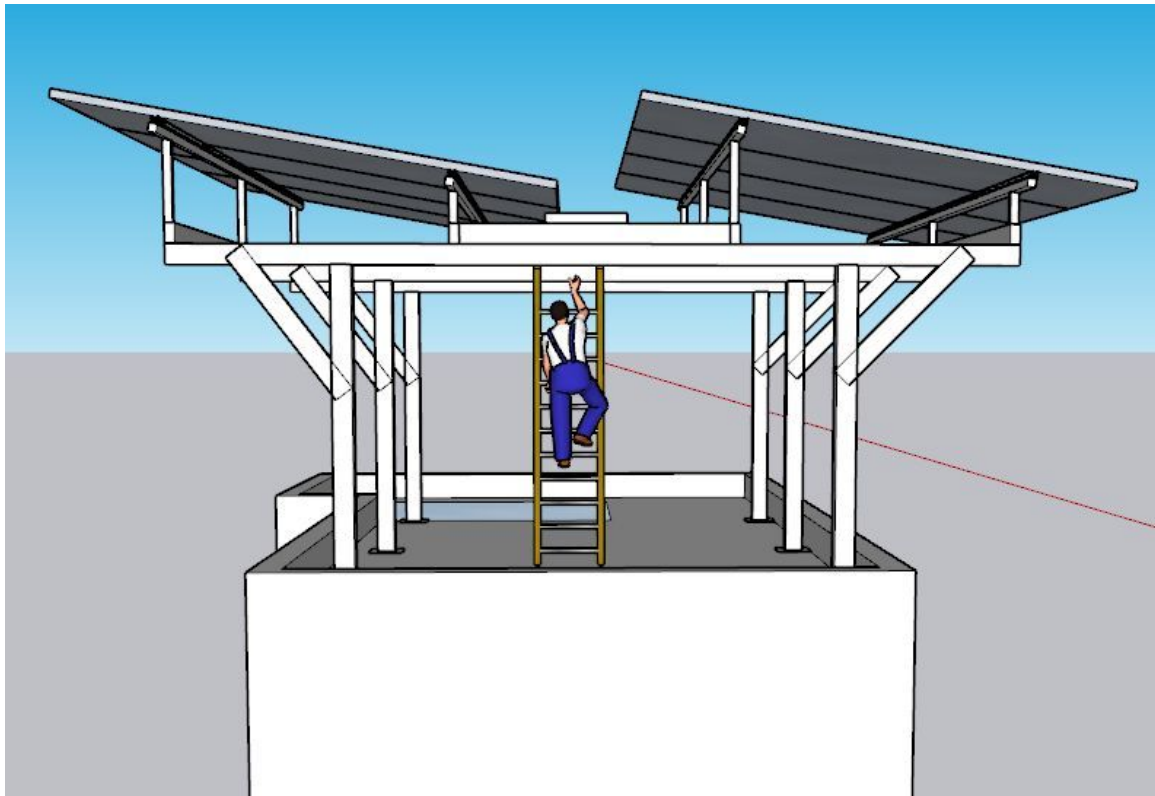
Side view (2)
