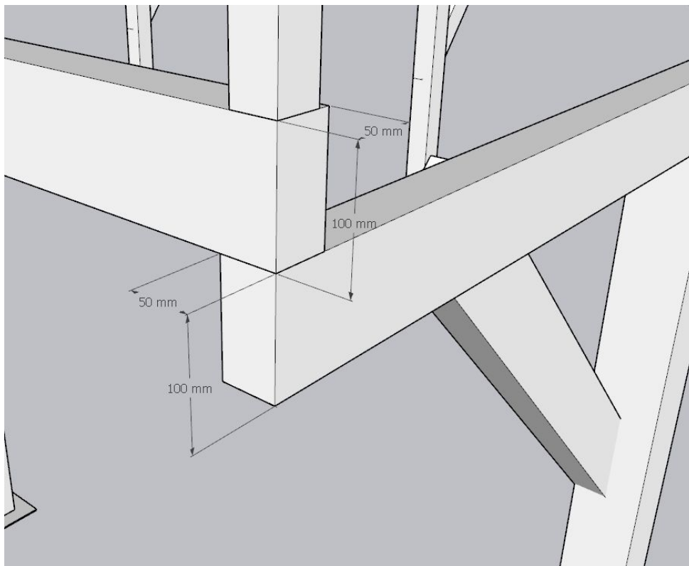
Structure details (3)
