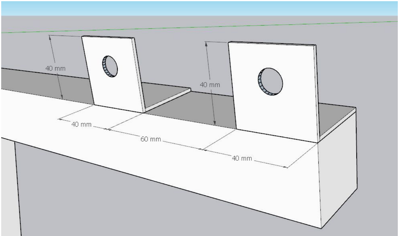
Structure details (8)
