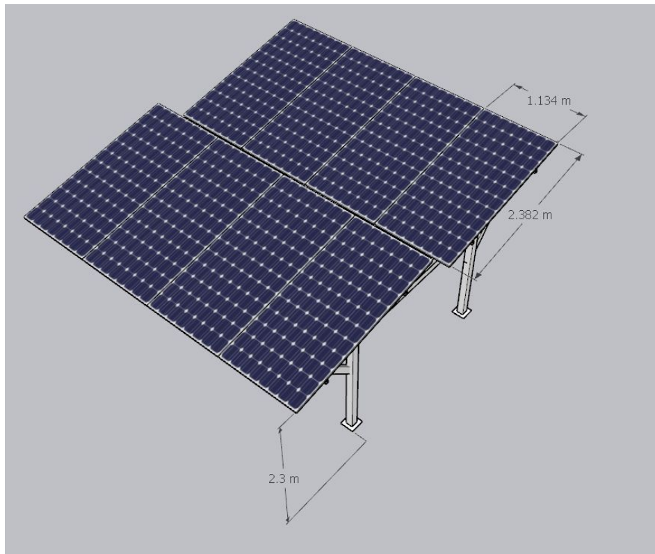
Panel dimensions
