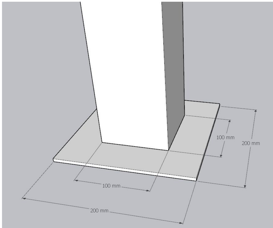
Structure details (6)
