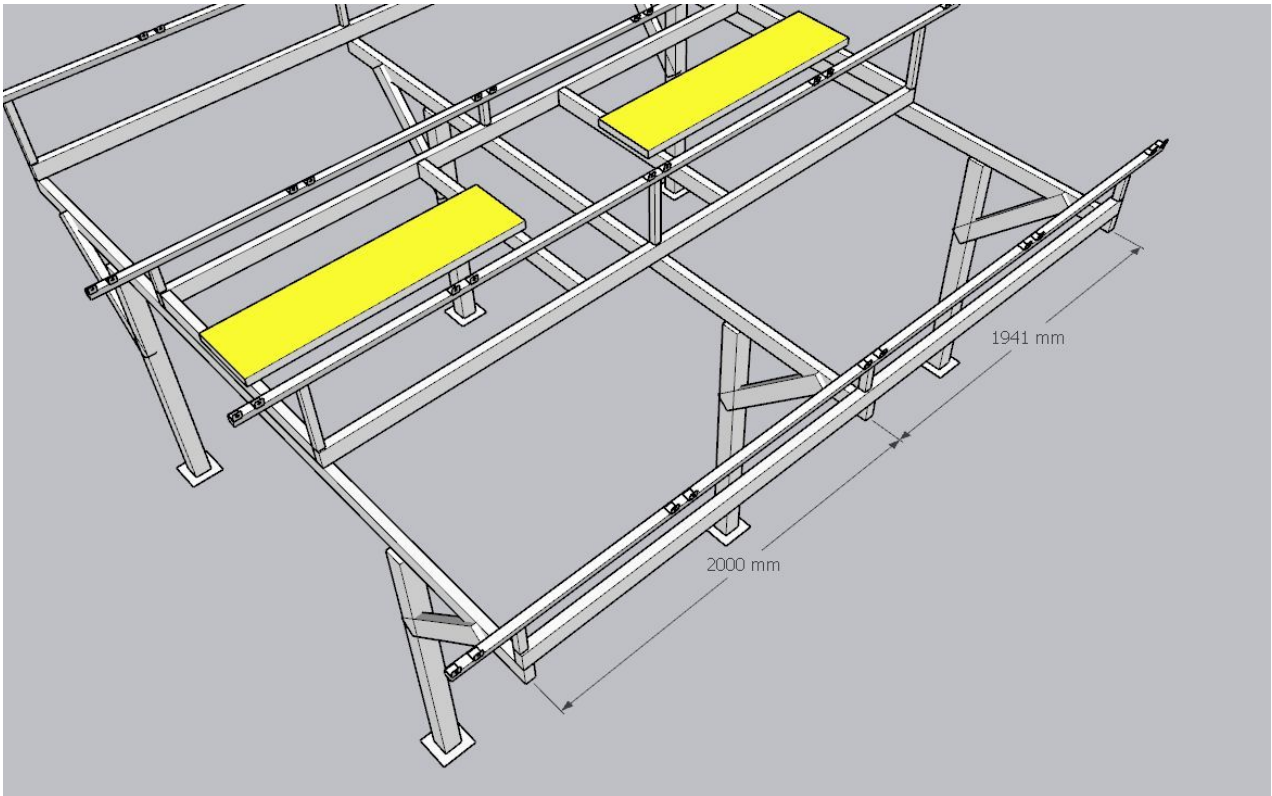
Structure details (4)
