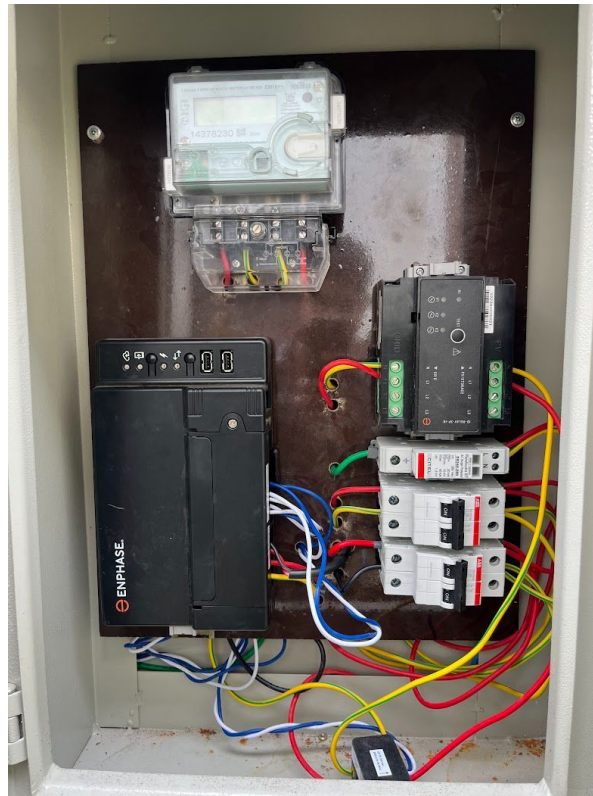
Existing Solar meter and Enphase accessories
