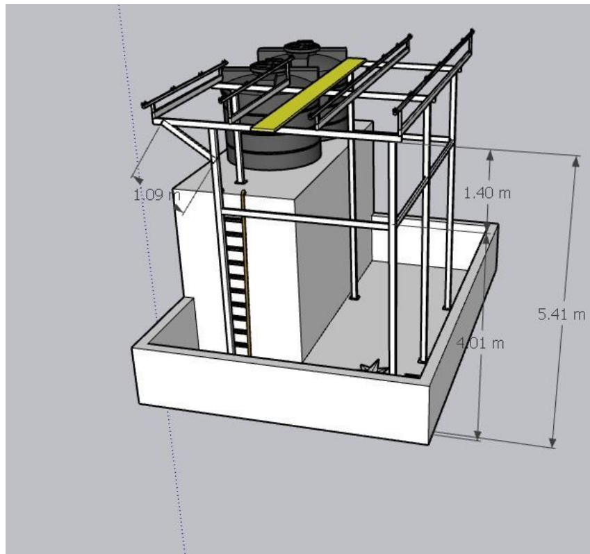
Structure details (9)
