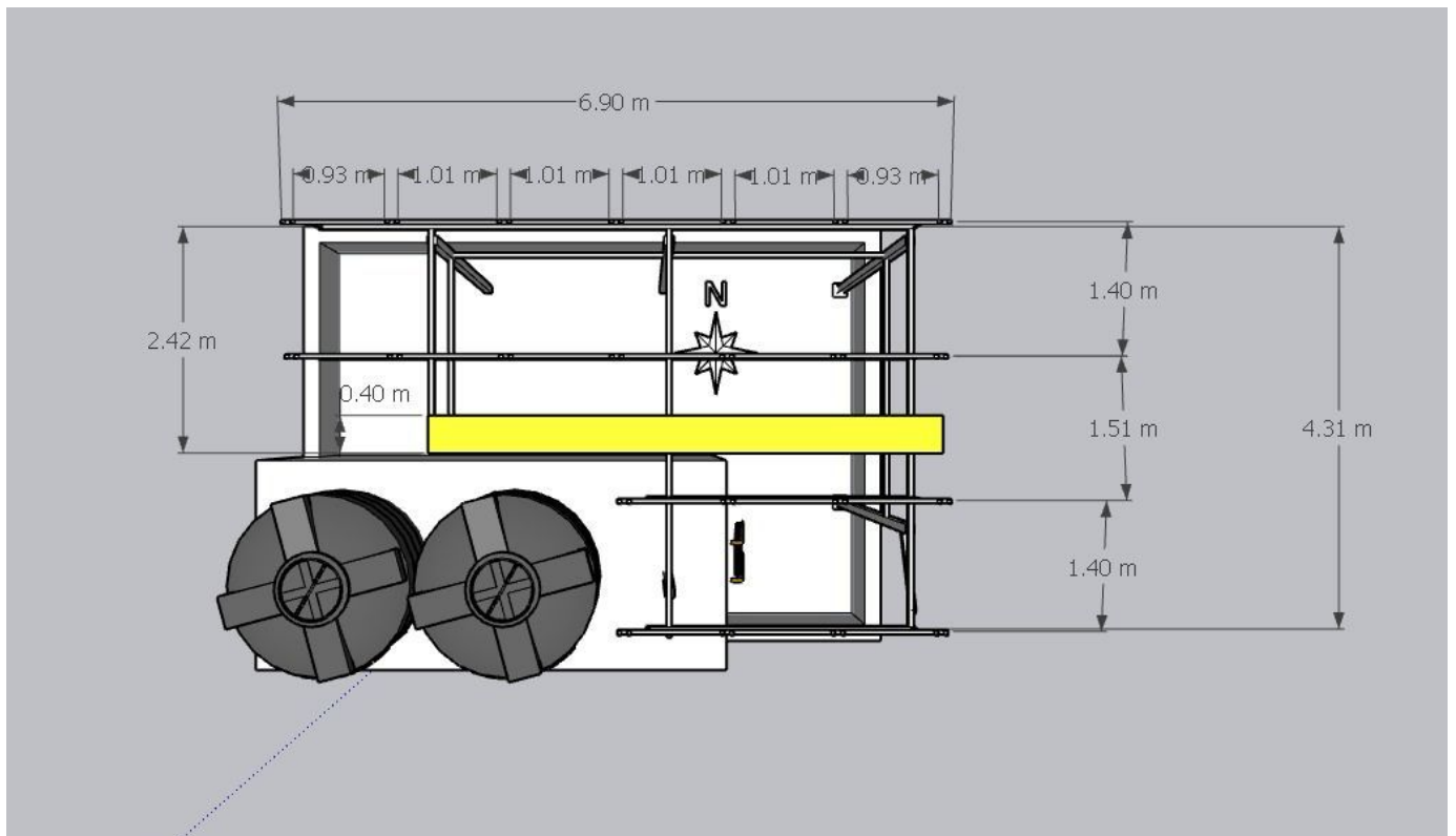
Structure details (1)
