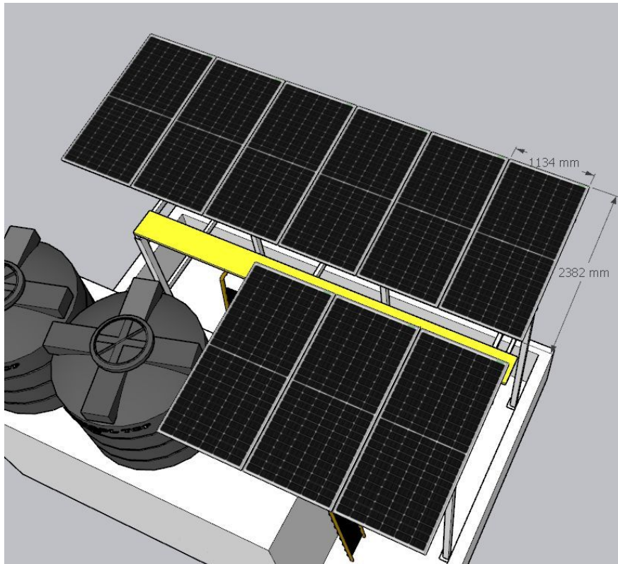
Panel dimensions
