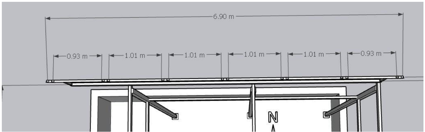
Structure details (2)
