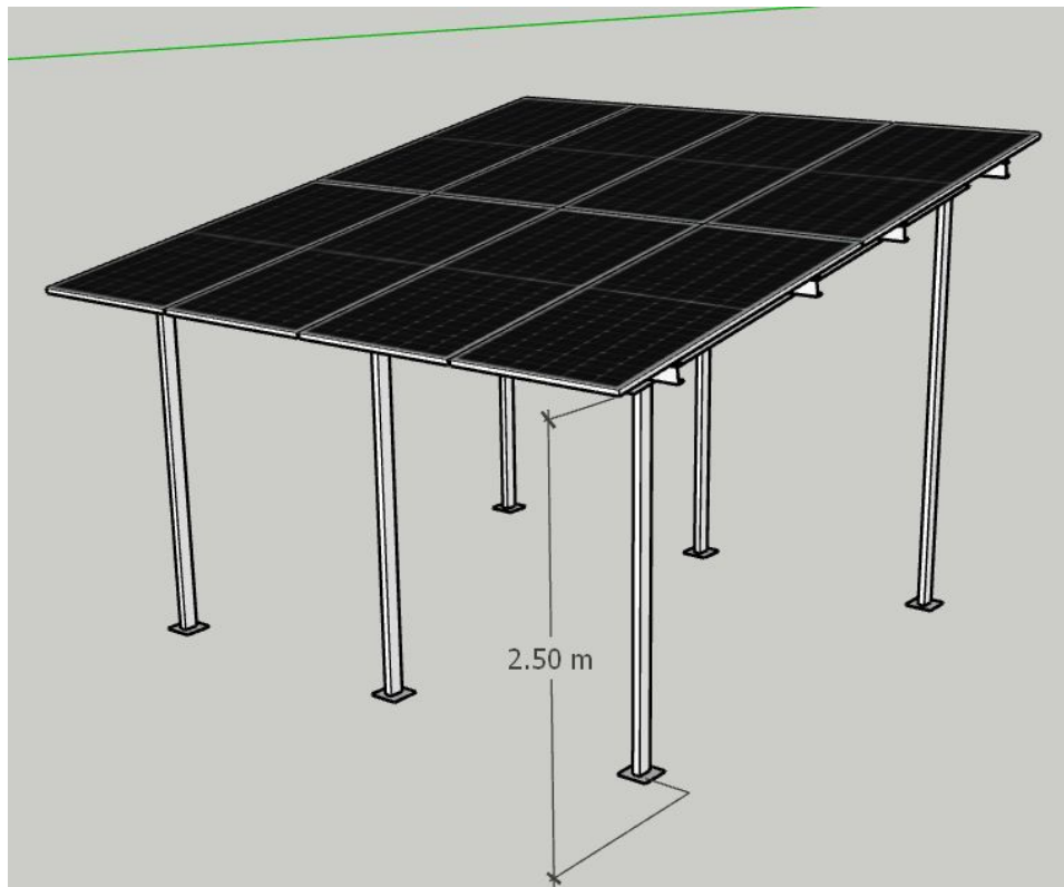
HDGI structure with 2.5m
