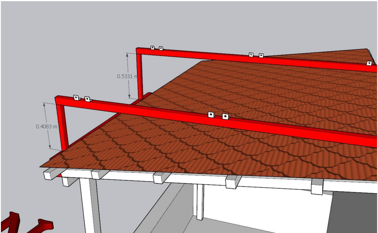
Structure details (3)
