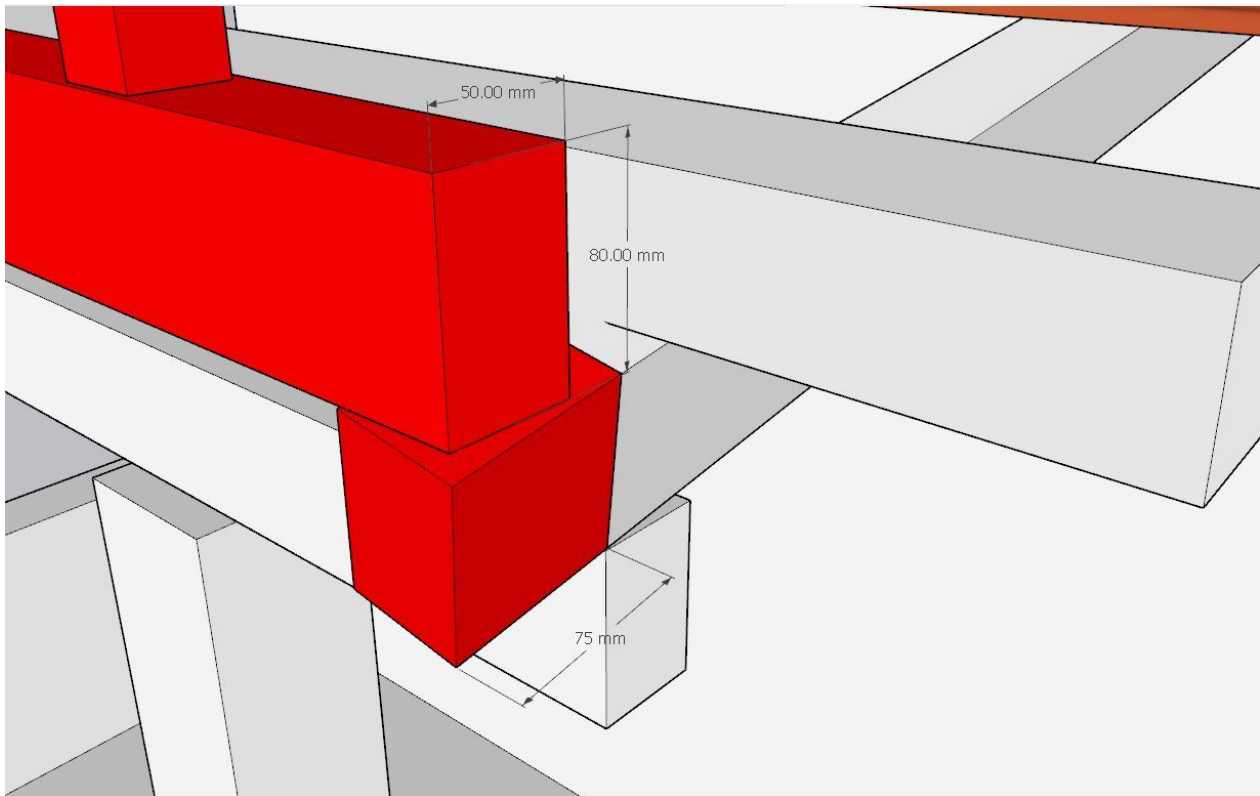
Structure details (5)
