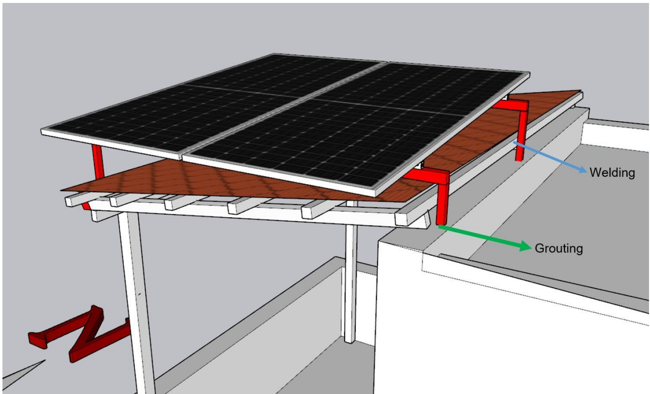
Structure details (7)
