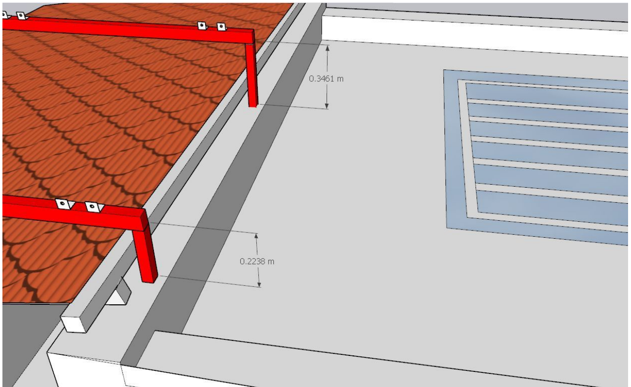
Structure details (4)
