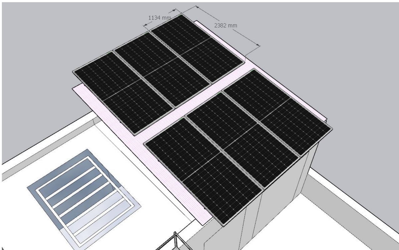
Panel dimension (1)
