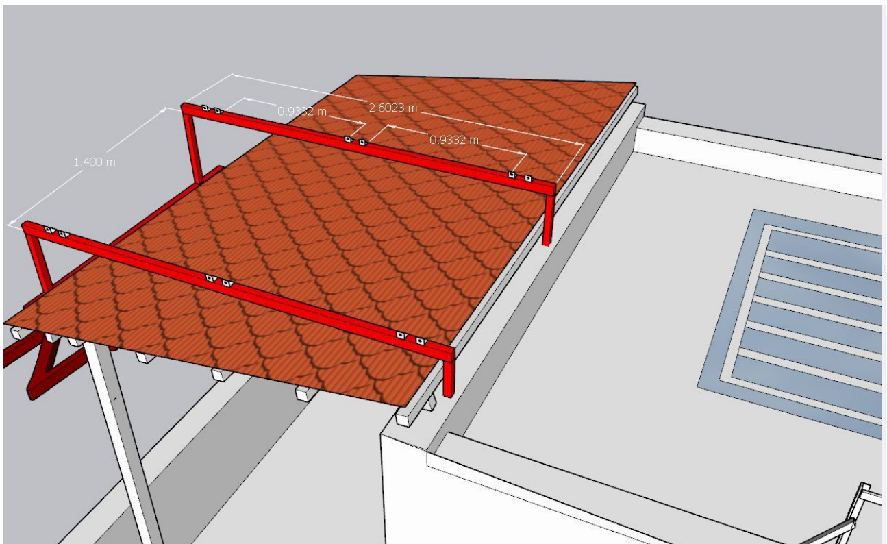
Structure details (2)
