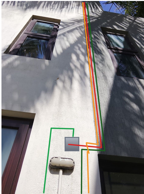
Make a hole to run the DC cable up to the inverter location.
