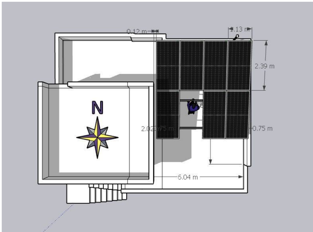
3. From September to December, between 02:00 and 04:30 Pm, the west side headroom wall will cast a shadow on the solar panels
