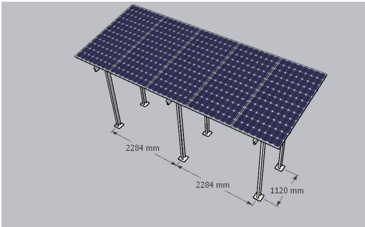
Structure details (2)
