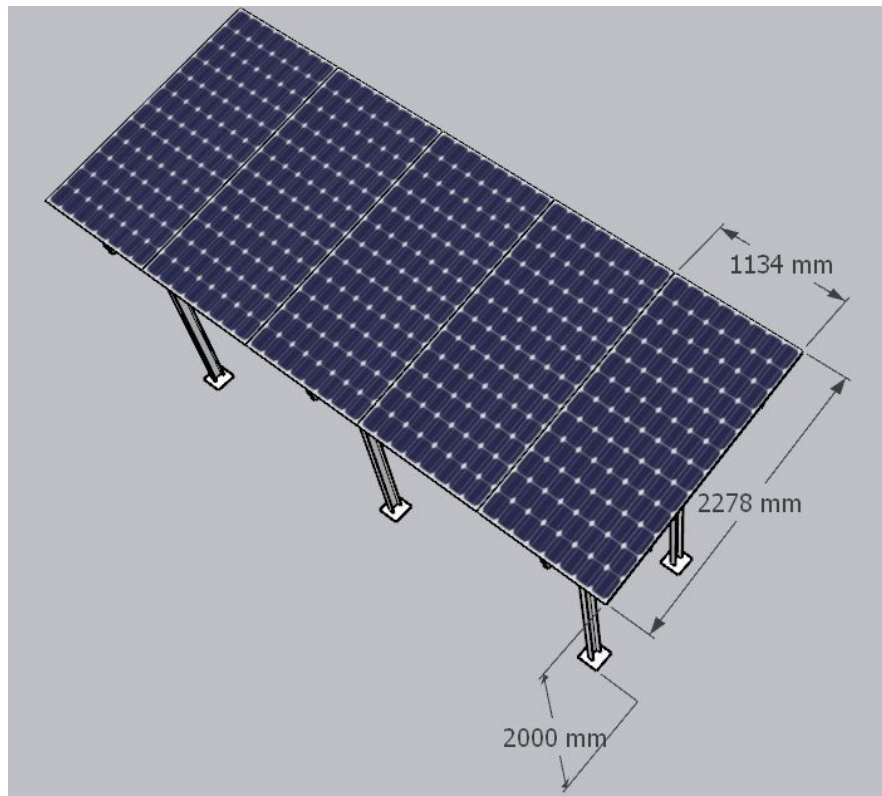
HDGI Structure (1P5 X 3 set of panels of Waaree DCR bifacial 585 Wp)
