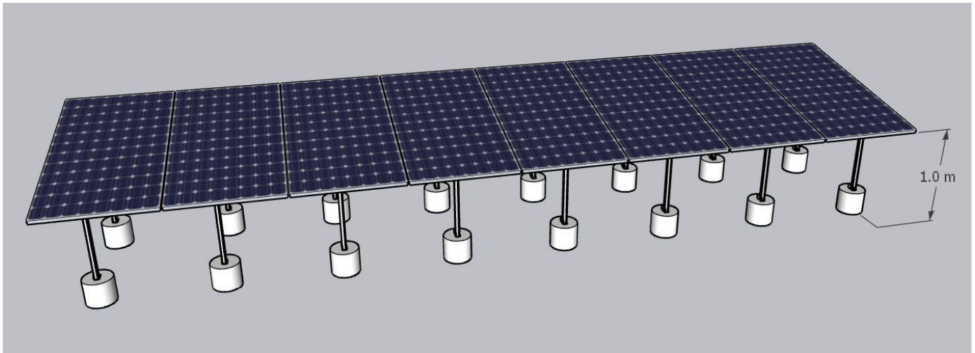
8P1 Structure - 1no.
