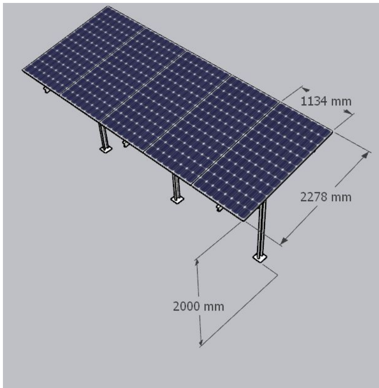
HDGI Structure (1P5 X 1 set of panels of Waaree DCR bifacial 585 Wp)
