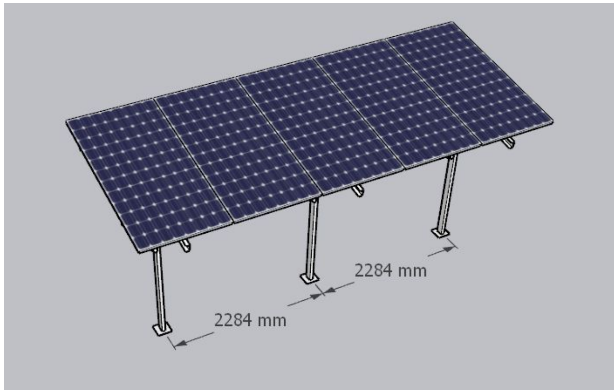
Structure details (2)
