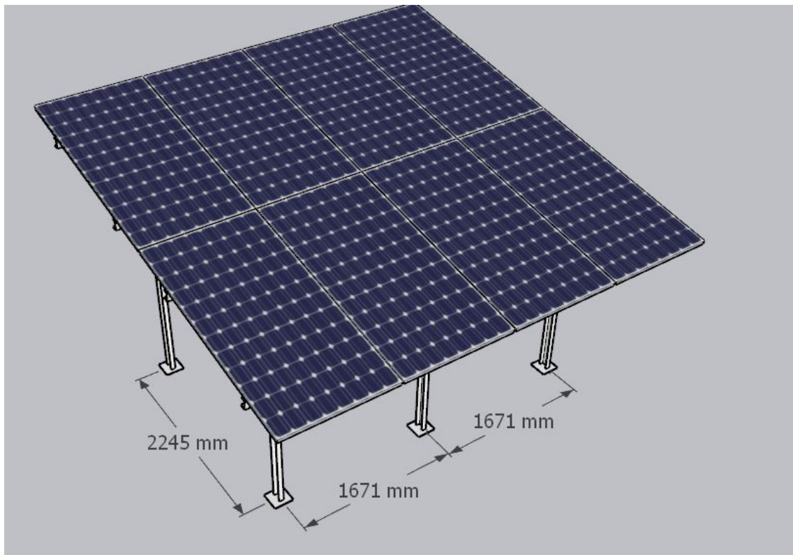
Structure details (1)
