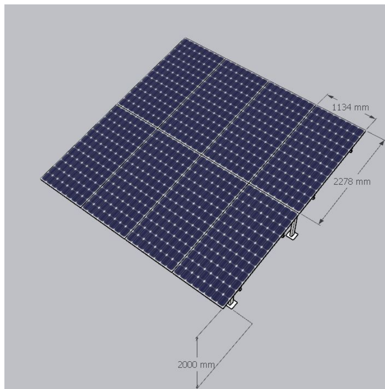
HDGI Structure (2P4 X 5 set of panels of Waaree DCR bifacial 585 Wp)
