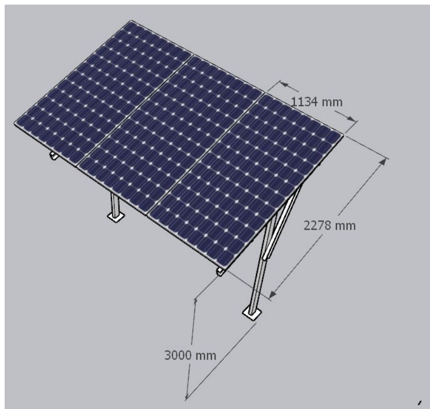
HDGI Structure (1P3 X 1 set of panels of Waaree DCR bifacial 585 Wp)
