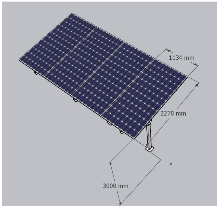
HDGI Structure (1P4 X 2 set of panels of Waaree DCR bifacial 585 Wp)
