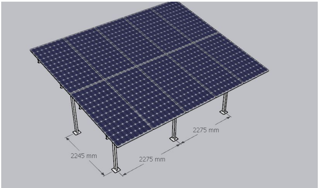
Structure details (5)
