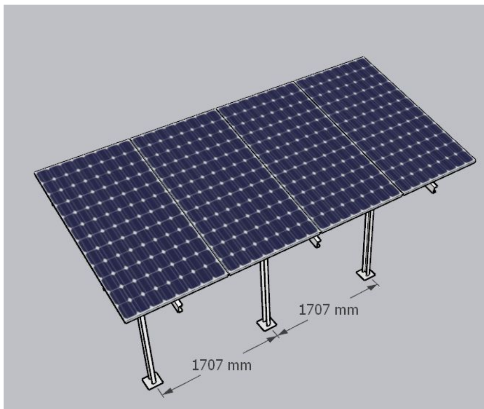
Structure details (7)
