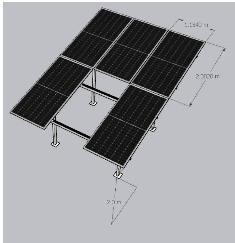
Panel dimensions
