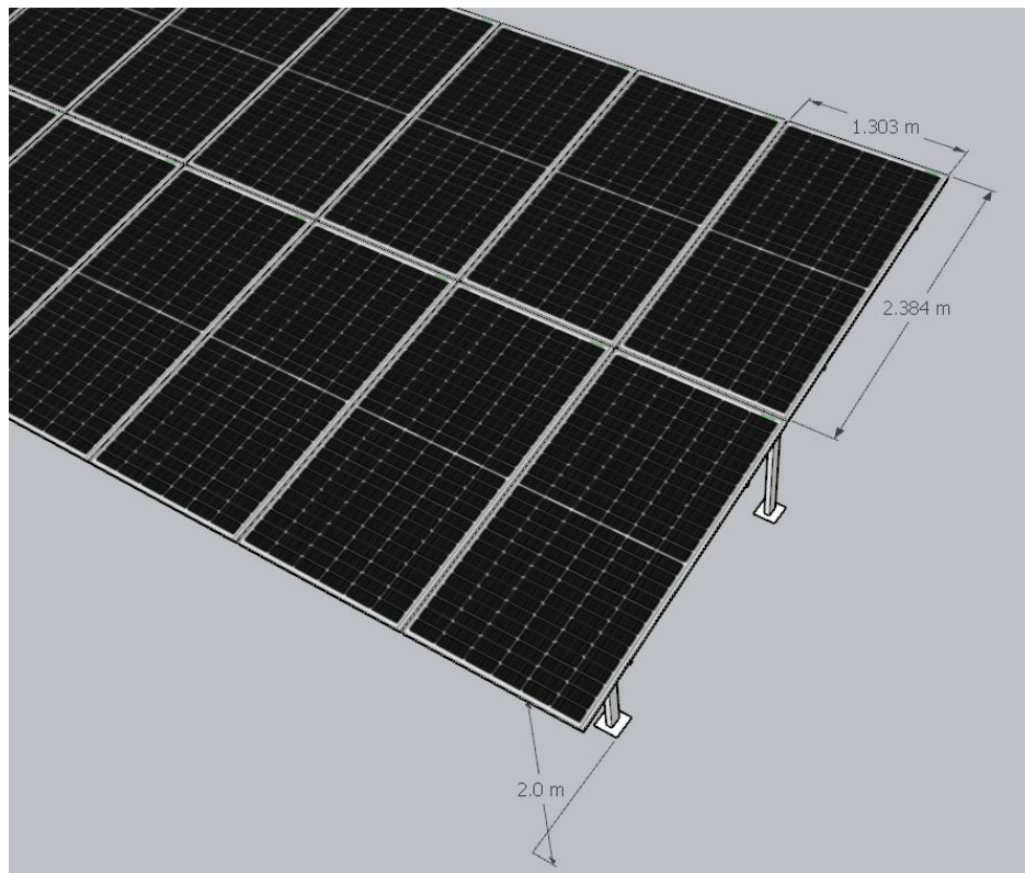
Panel dimensions
