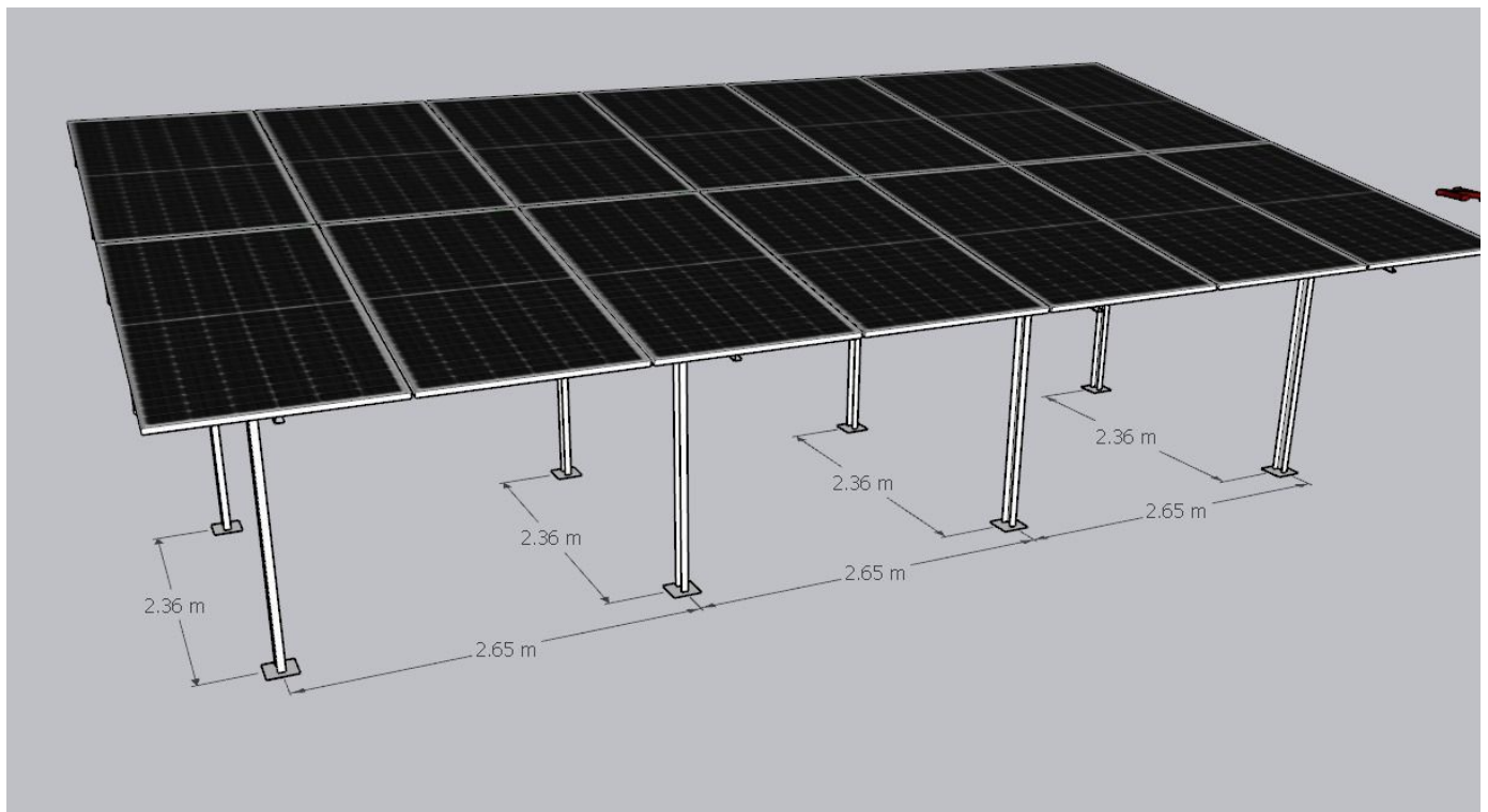
Structure details (2)
