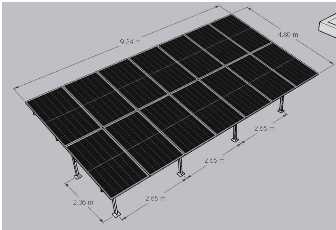
Structure details (1)
