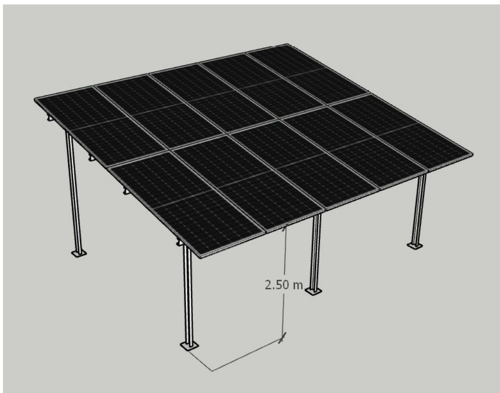
5P2 HDGI structure with 2.5m height - 2No.s
