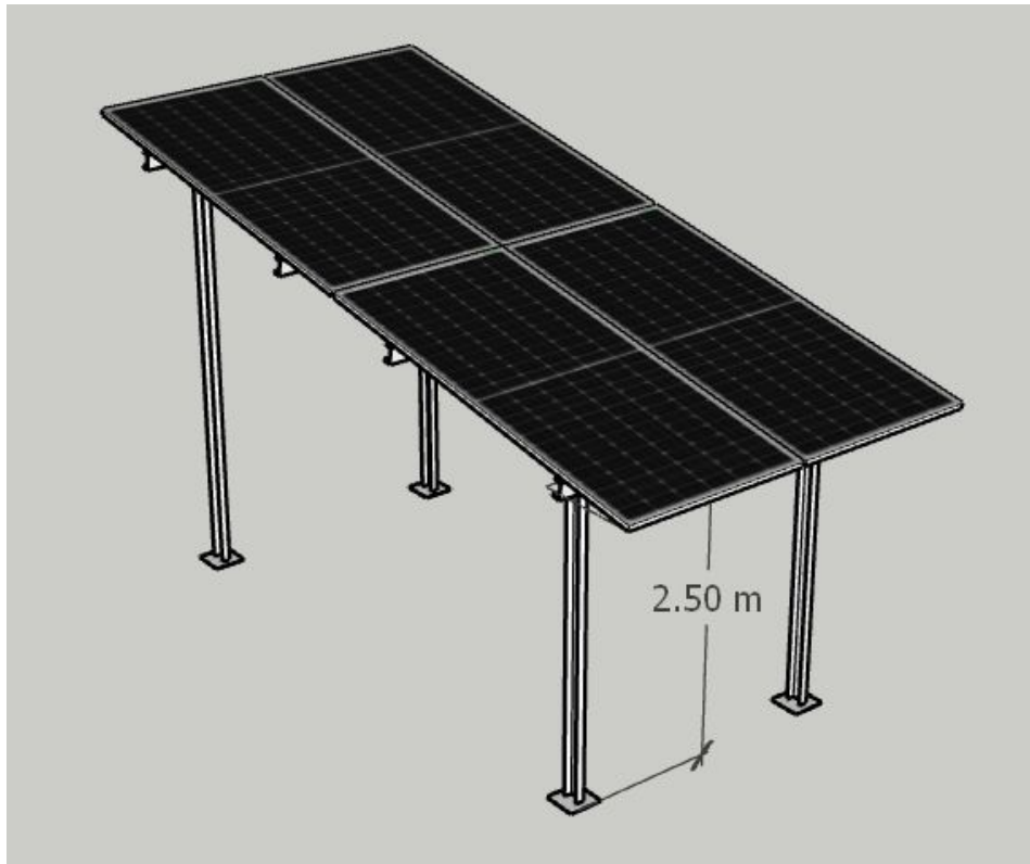
2P2 HDGI structure with 2.5m height - 1No.
