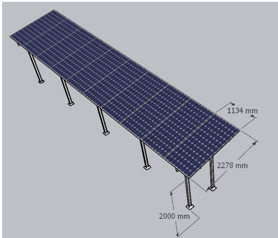
HDGI Structure (1P10 X 1 set of panels of Waaree DCR bifacial 585 Wp)
