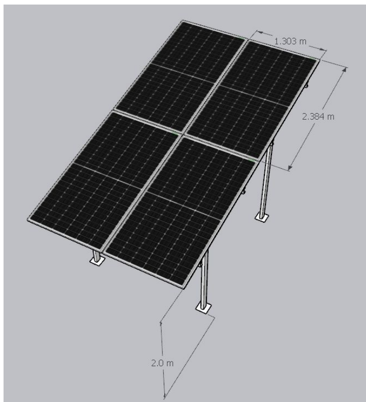
Panel dimensions (1)
