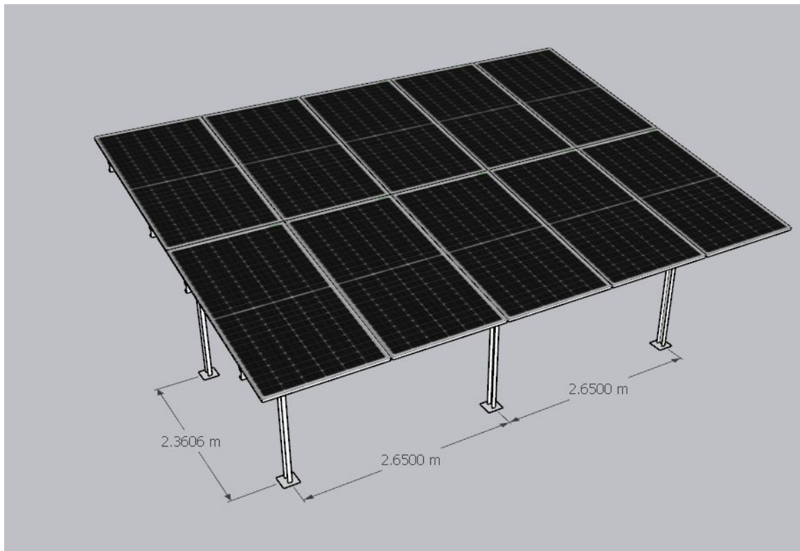
Structure details (2)
