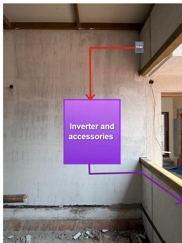
AC cable from Inverter to termination area is under customer scope.
