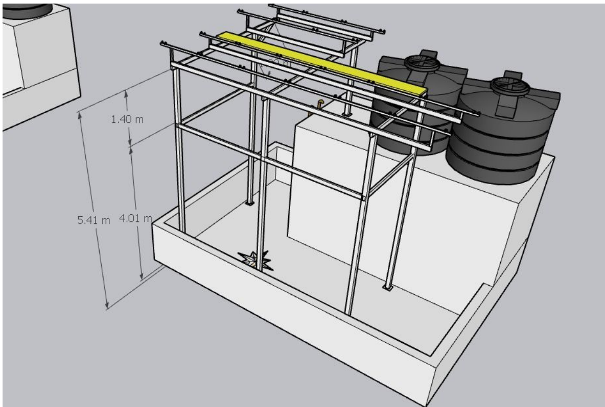
Structure details (7)
