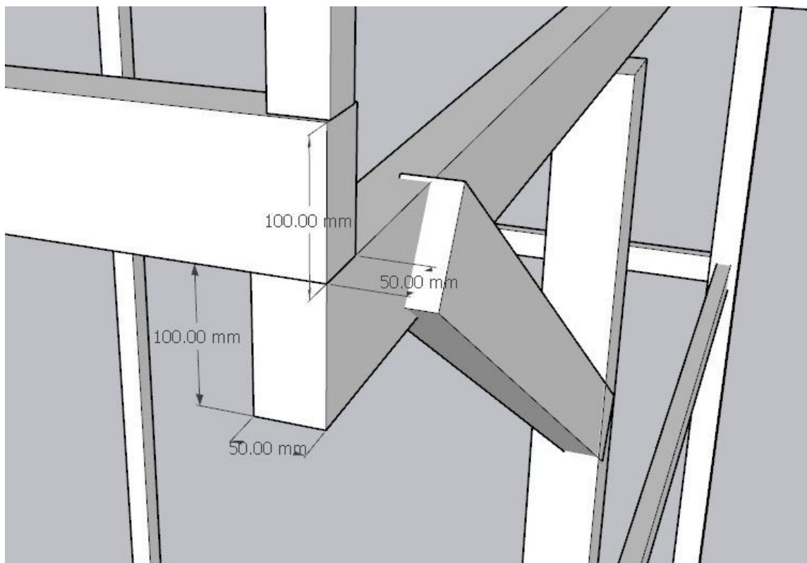
Structure details (11)
