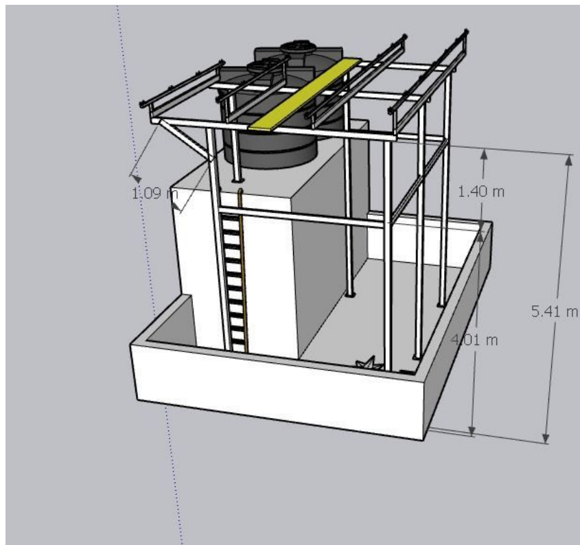
Structure details (9)
