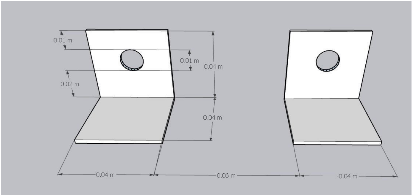
Structure details (6)
