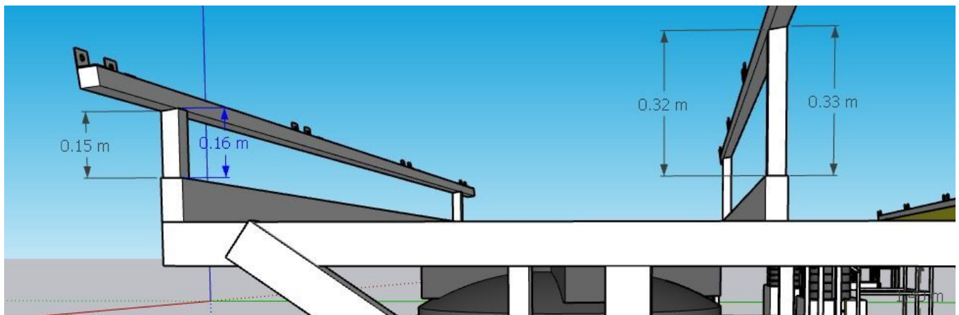
Structure details (5)
