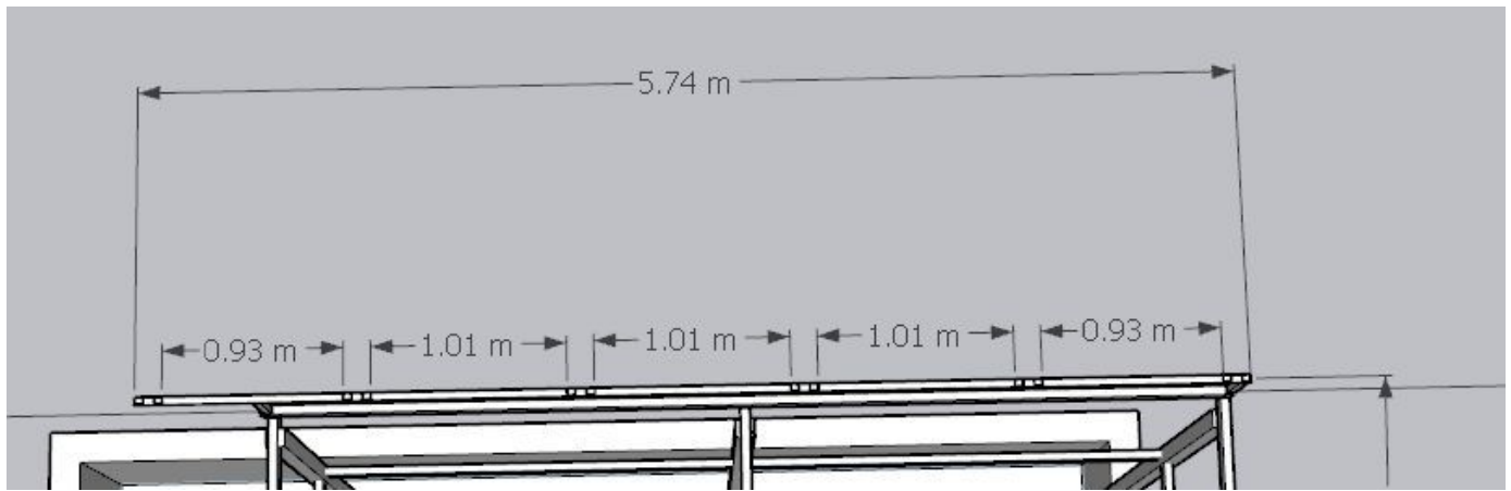
Structure details (3)
