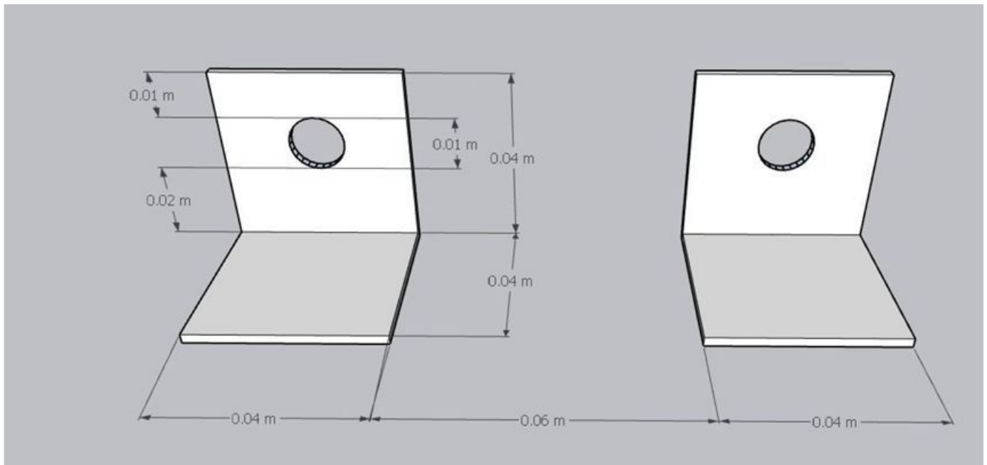
Structure details (2)
