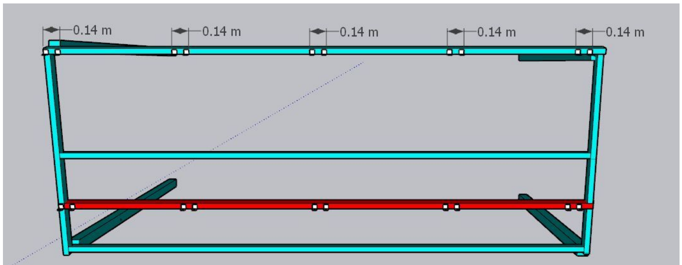
Structure details (1)
