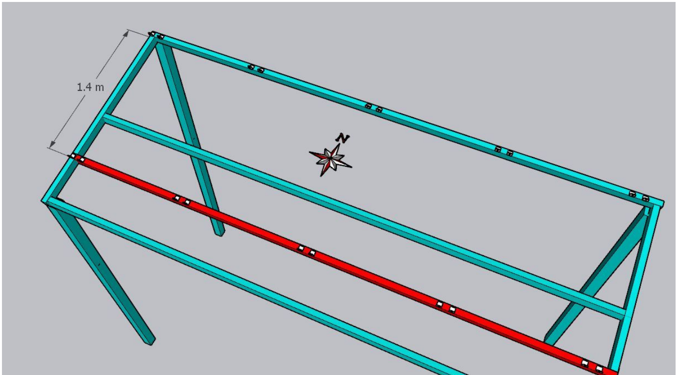
Structure details (3)
