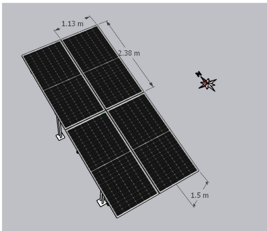
Panel dimensions
