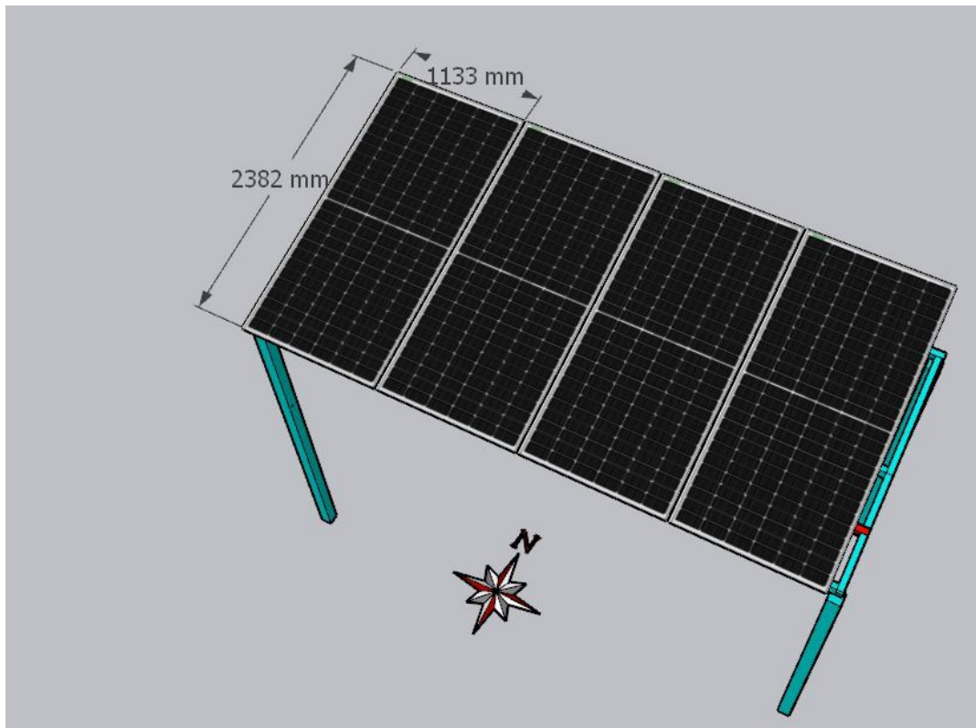
Panel dimensions
