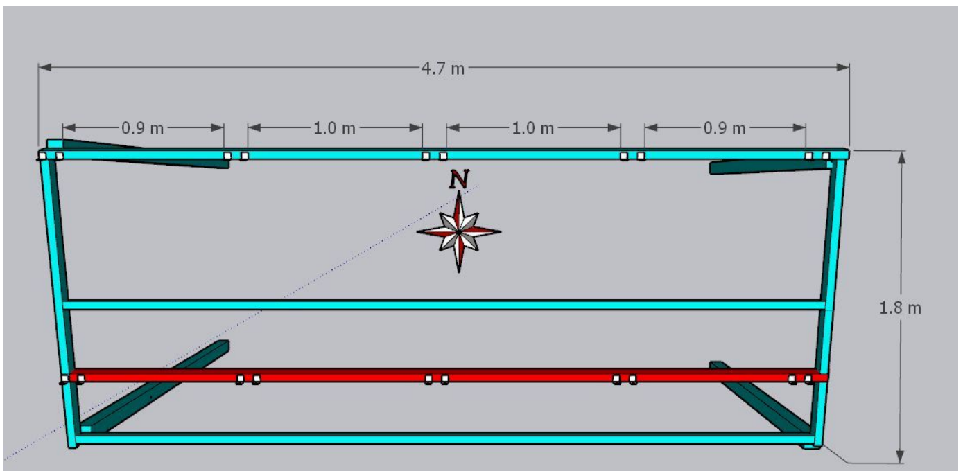
Structure details (4)
