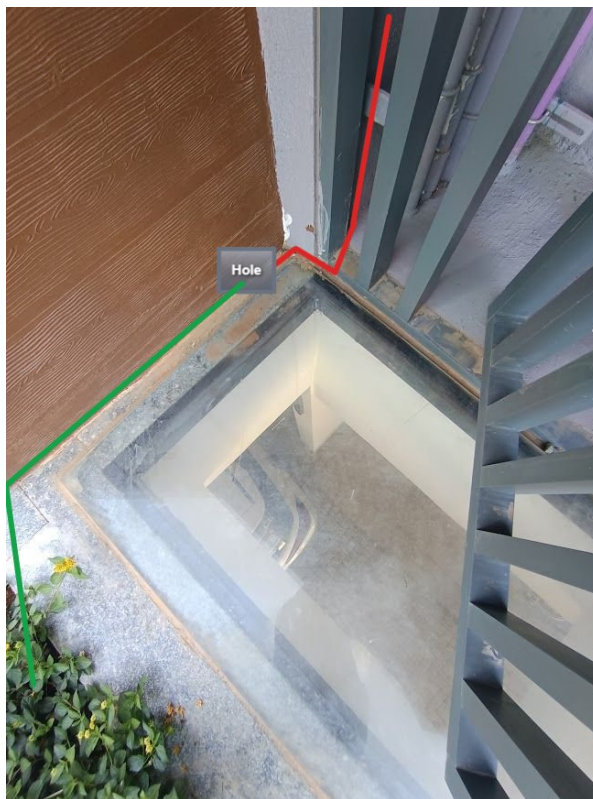
One hole has to be made to run the DC and AC cables
