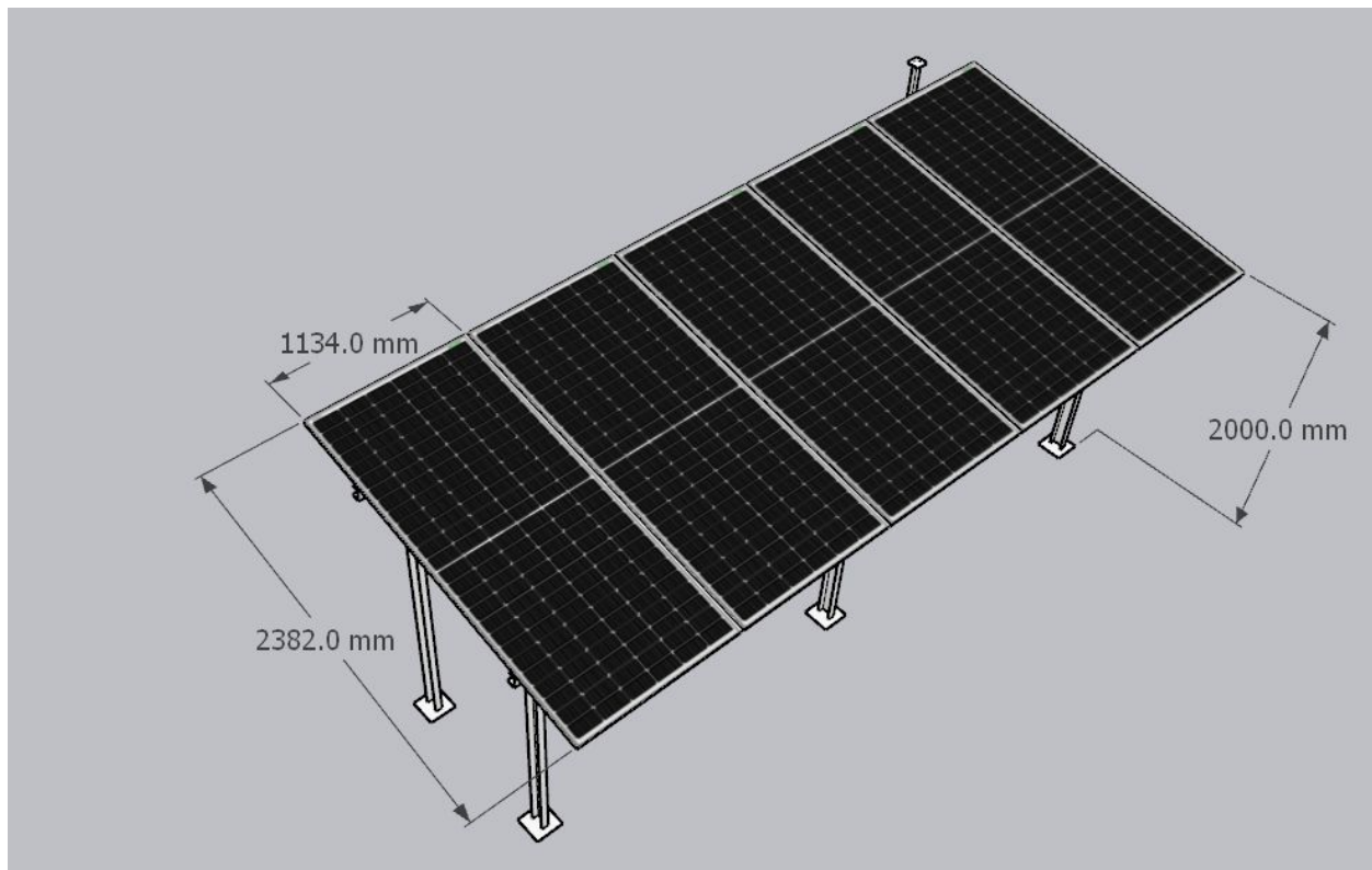
Panel dimension
