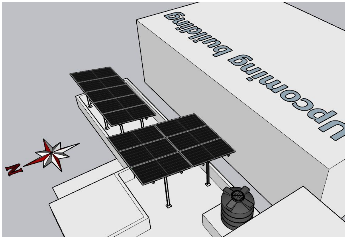
Side view (1)
