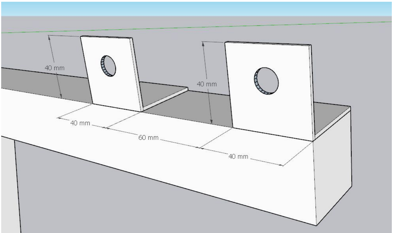
Structure details (8)
