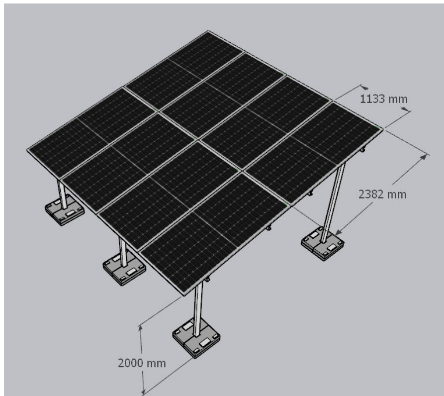
Panel dimensions
