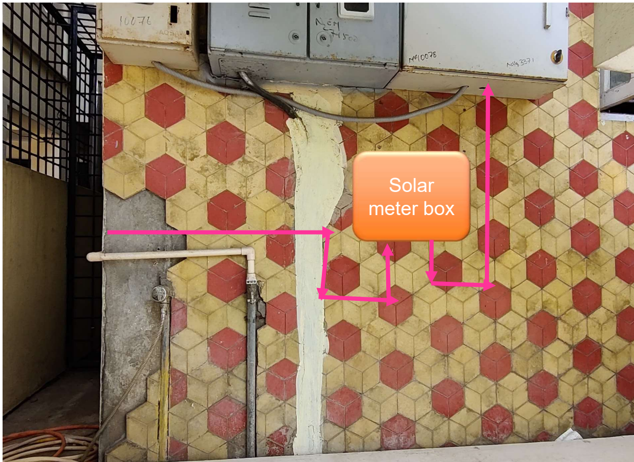
AC cable running on the parapet wall south side of the building till the solar meter box
