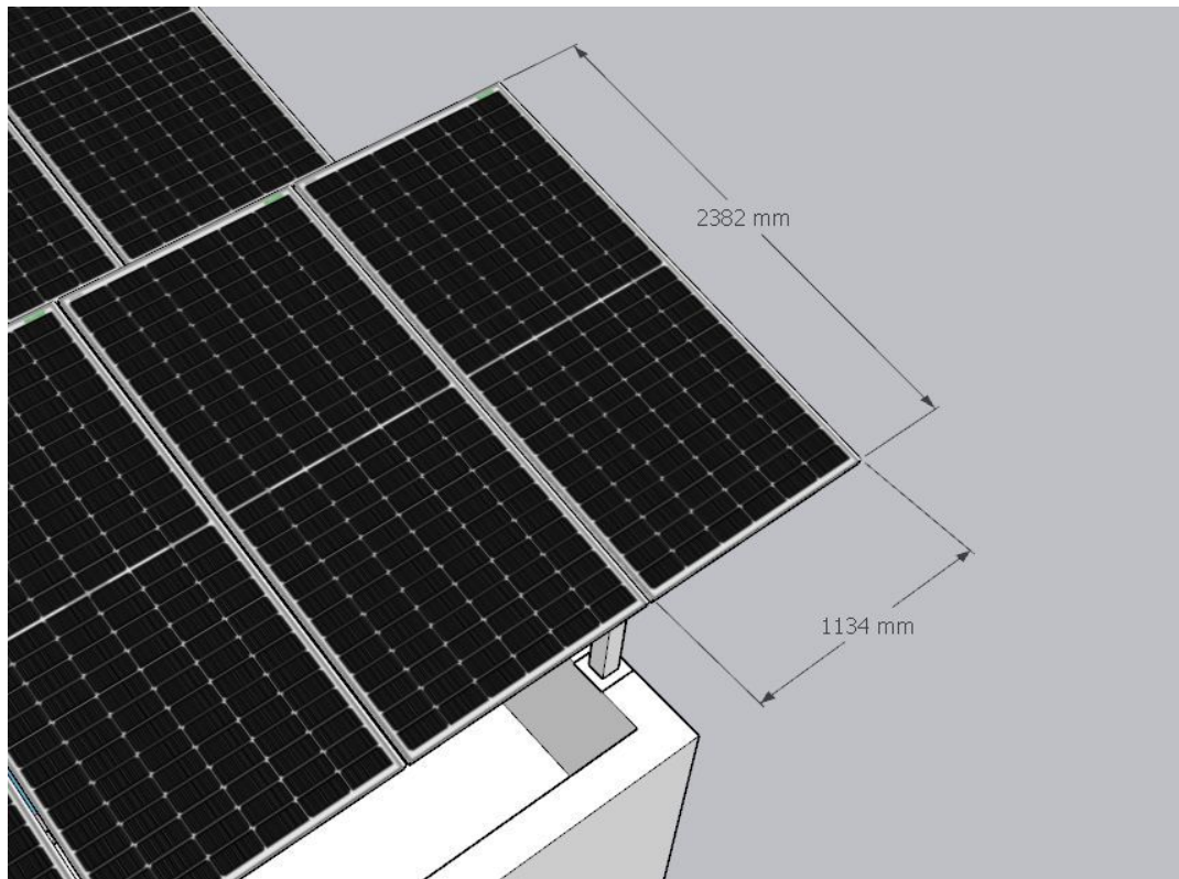
Panels dimensions
