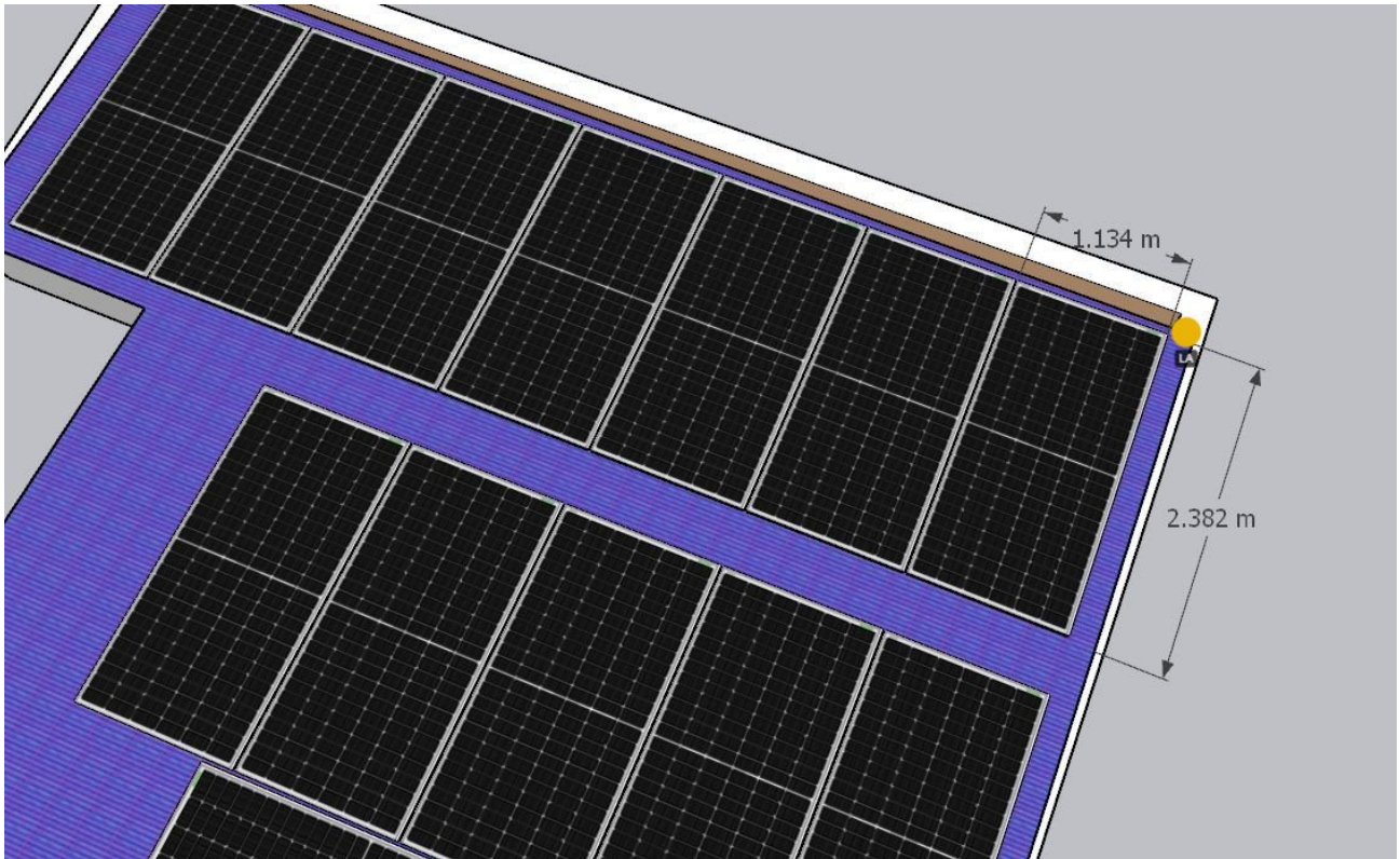
Panel dimensions (1)
