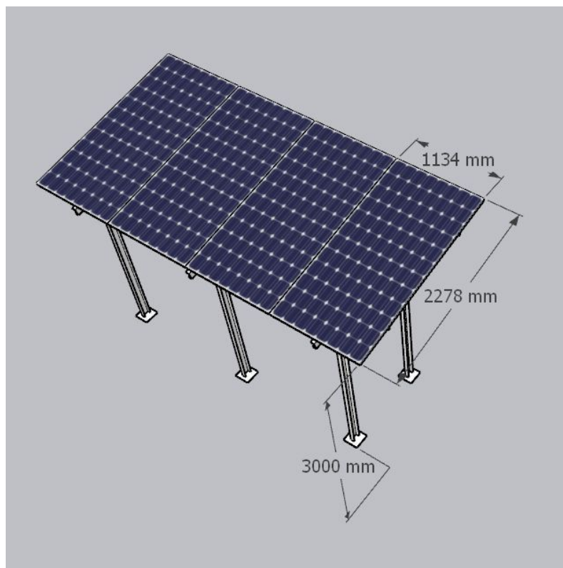
HDGI Structure (1P4 X 2 set of panels of Waaree DCR bifacial 585 Wp)
