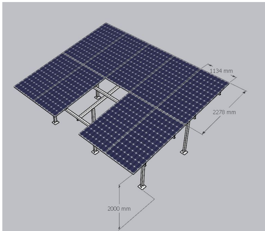
HDGI Structure (2P5 X 1 set of panels of Waaree DCR bifacial 585 Wp)
