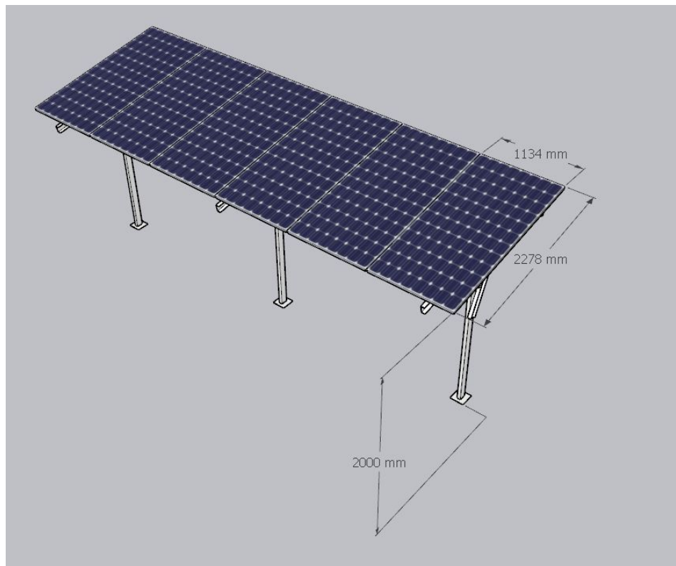
HDGI Structure (1P6 X 1 set of panels of Waaree DCR bifacial 585 Wp)
