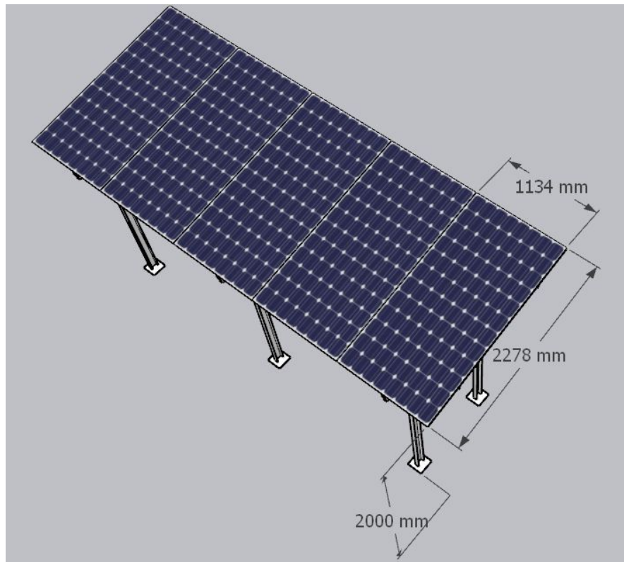
HDGI Structure (1P5 X 2 set of panels of Waaree DCR bifacial 585 Wp)
