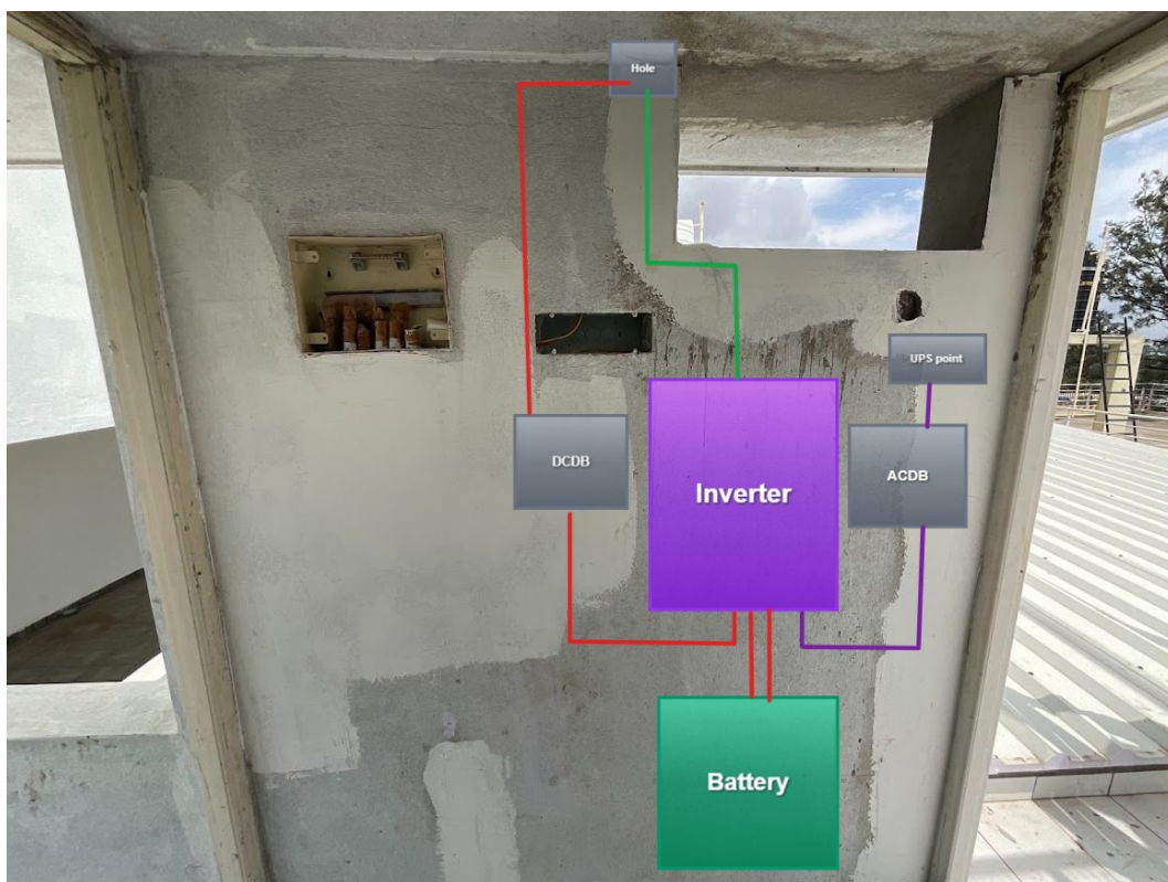
One hole has to be made to run the cables
