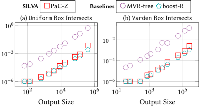
Figure 14: Box intersects query on synthetic datasets, lower the better. All axes are in log scale. All queries are read-only and can be parallelized.
