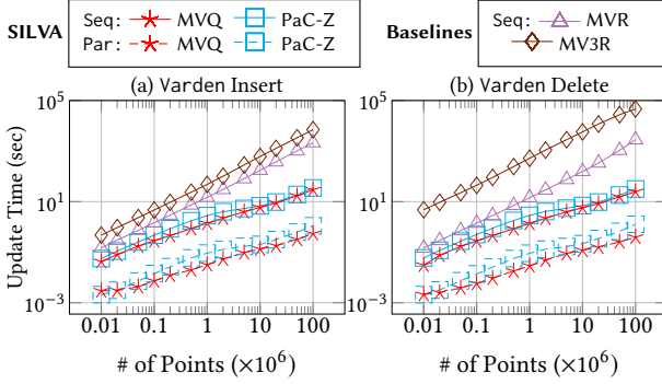
Figure 7: Batch update evaluation on Varden with 100M points, lower is better (log scale). Dashed lines are running in parallel (96 cores).
