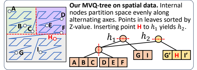
Figure 3: MVQ-tree Example. MVQ-tree directly applies path-copying to classic quadtrees. Unmodified regions (e.g., the upper part in the figure) are shared across versions.
