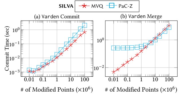
Figure 8: Commit and Merge time on Varden with 100M points, lower is better. Modification consists of 50% insertion and 50% deletion.
