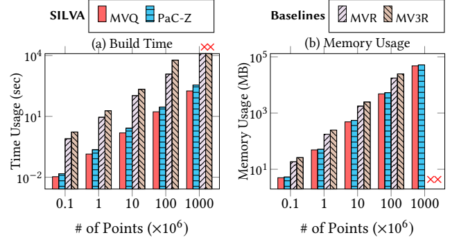
Figure 6: BUILD time (Sequential) and memory evaluation on Varden dataset, lower is better (log-scale). \times means timeout or not applicable.
