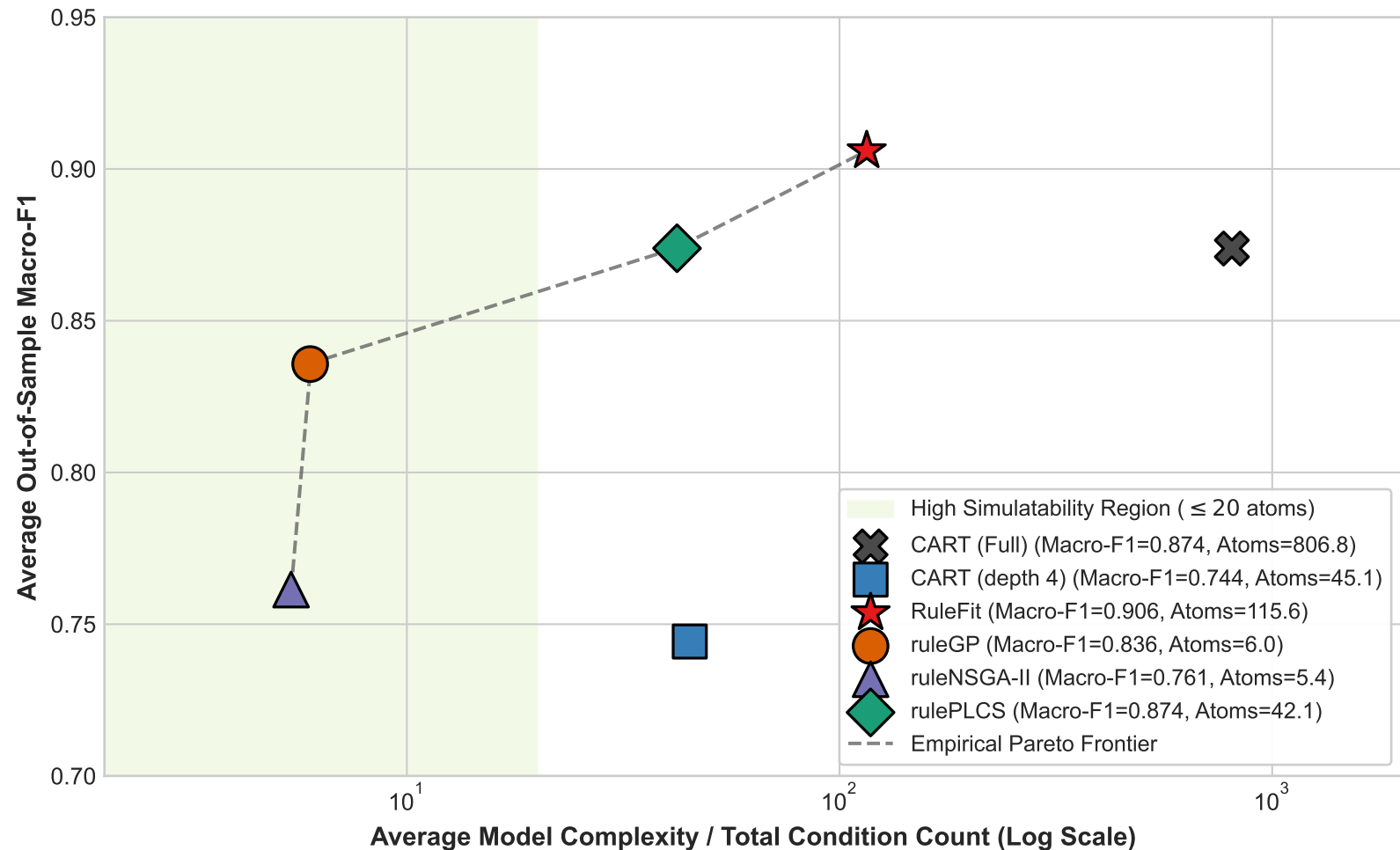
Pareto Trade-off: Classification Predictive Performance vs. Model Complexity
