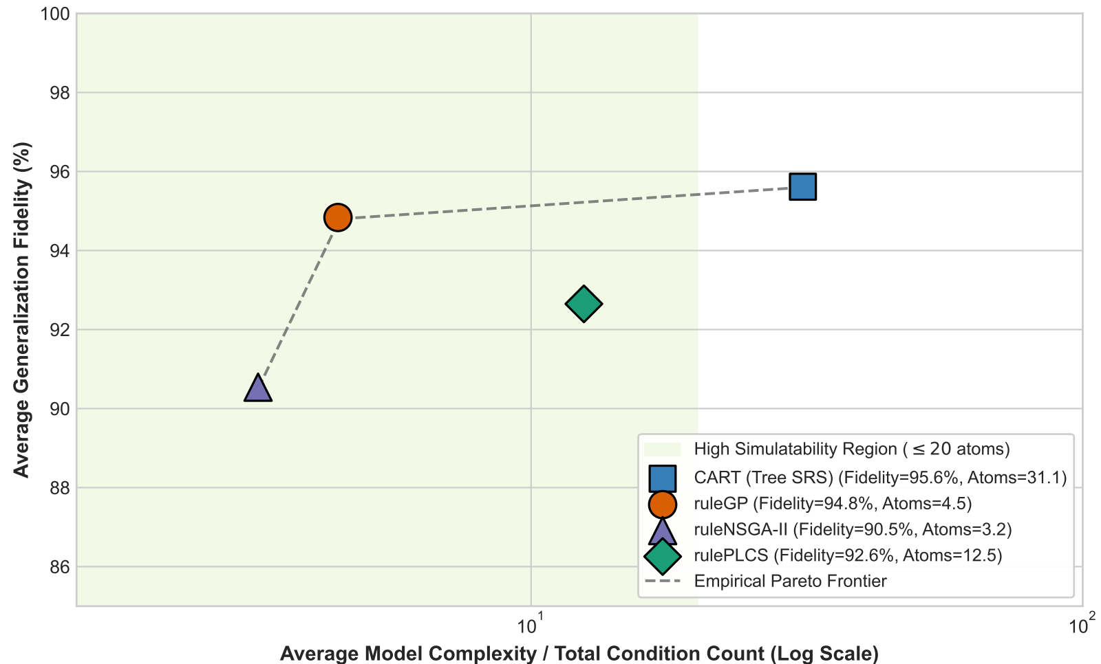
Pareto Trade-off: Cluster Explanation Fidelity vs. Model Complexity
