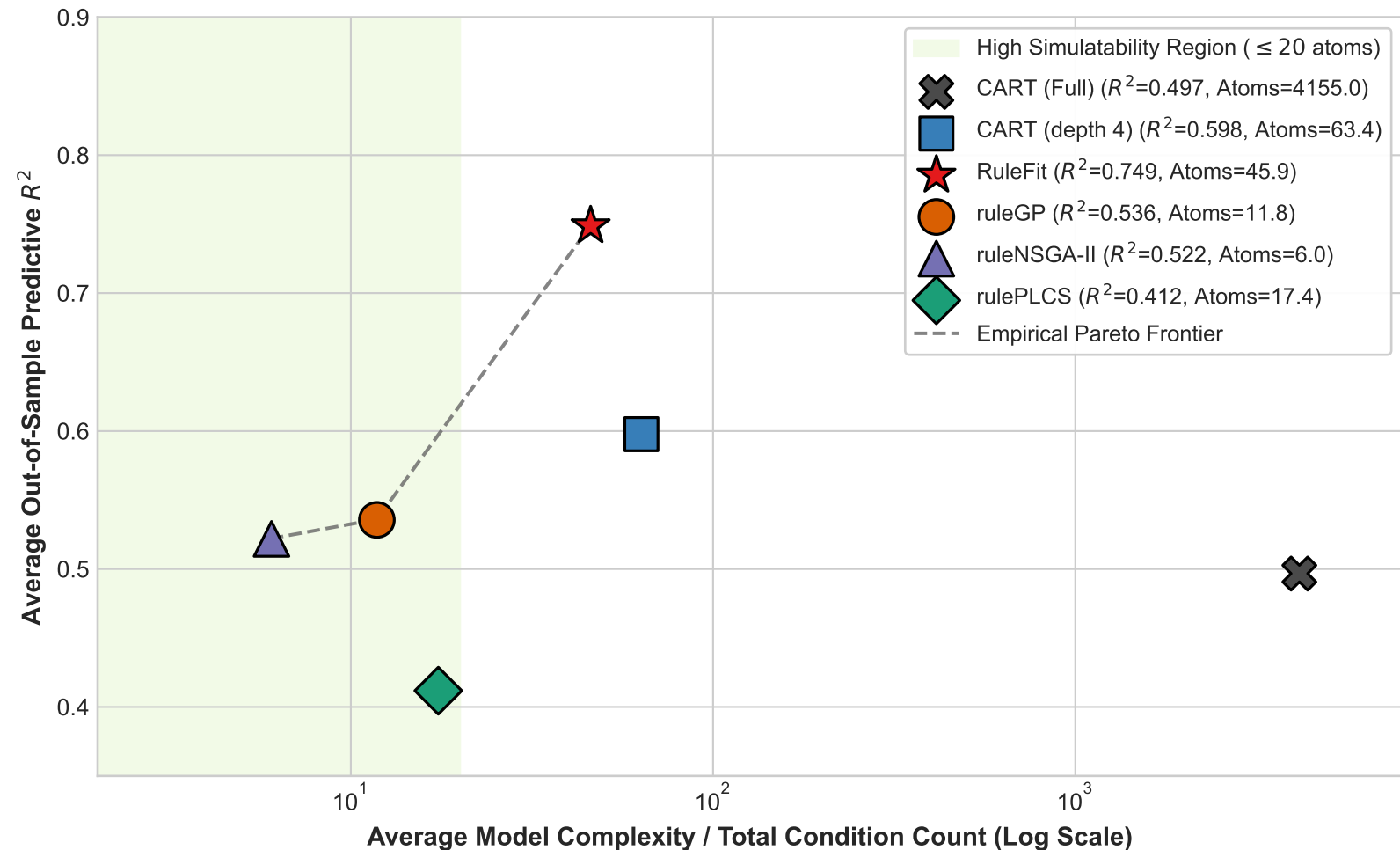
Pareto Trade-off: Continuous Regression Accuracy vs. Model Complexity
