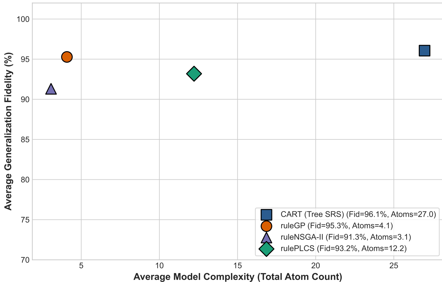
Pareto Trade-off: Cluster Explanation Fidelity vs. Complexity
