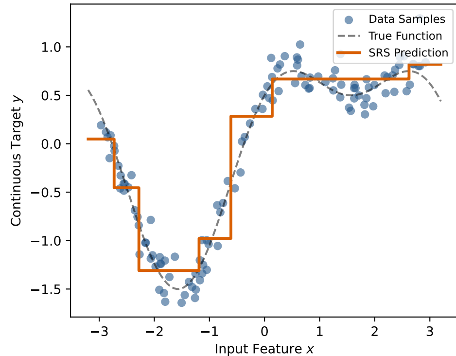
ruleNSGA-II (SRS Regressor) R^2=0.93 | Rules=8 | Atoms=12
