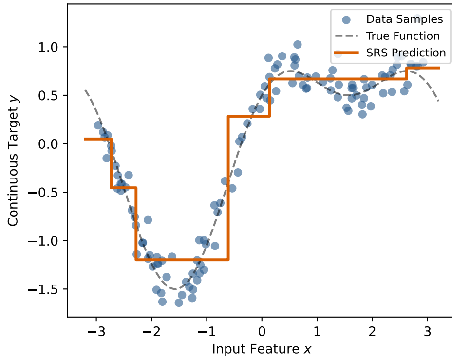
ruleGP (SRS Regressor) R^2=0.92 | Rules=6 | Atoms=9
