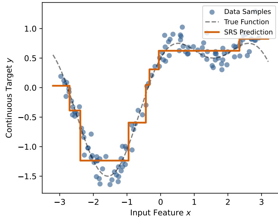
CART (Depth-3 SRS) R^2=0.95 | Rules=8 | Atoms=24
