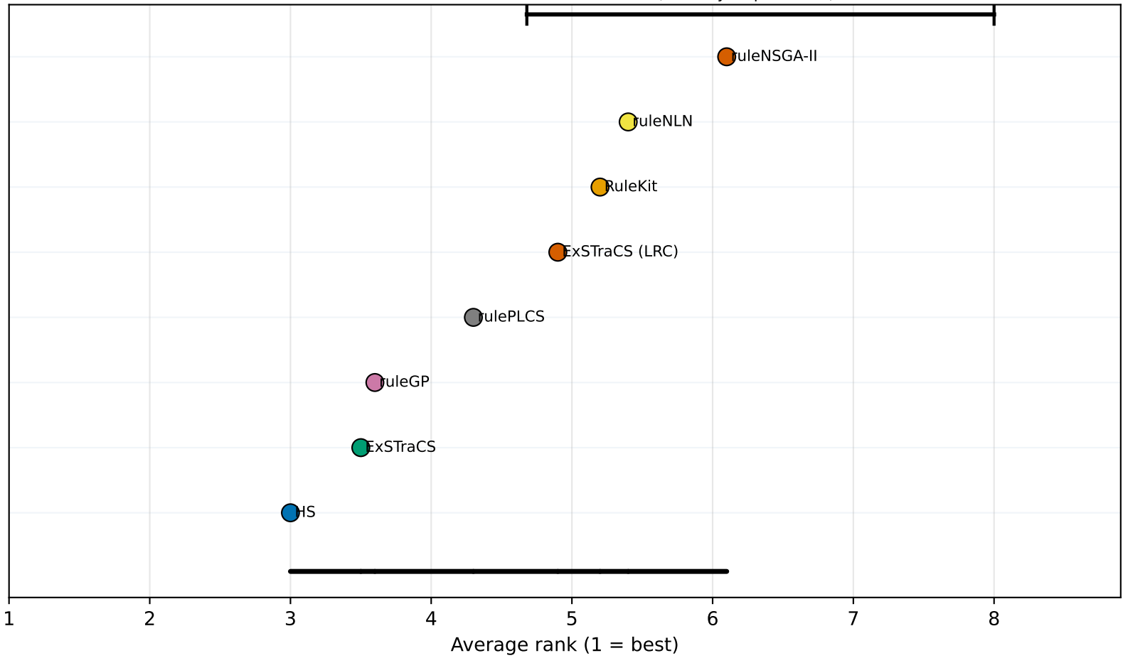
Critical Difference Diagram (F1 ranks across 10 datasets)
