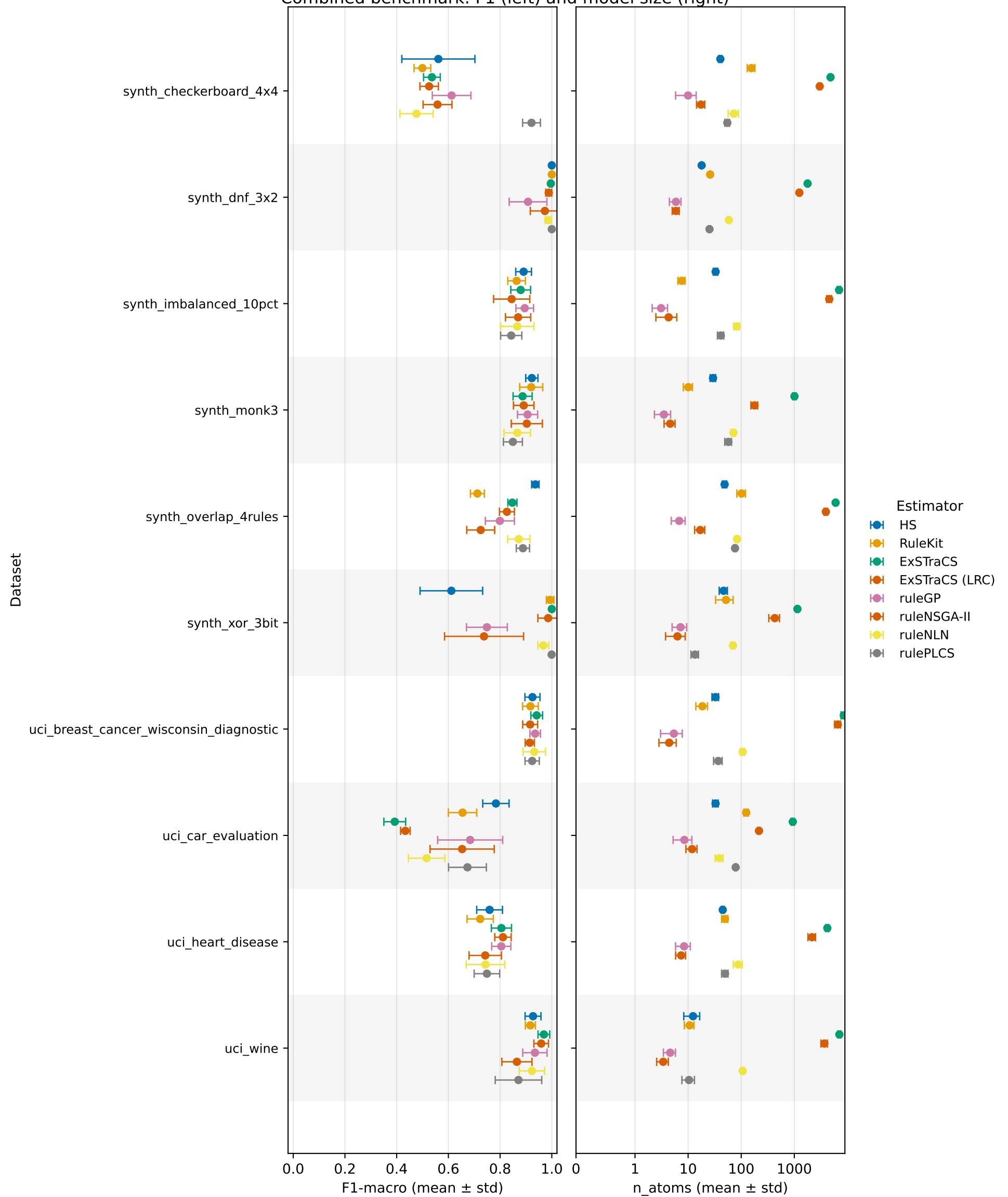
Combined benchmark: F1 (left) and model size (right)
