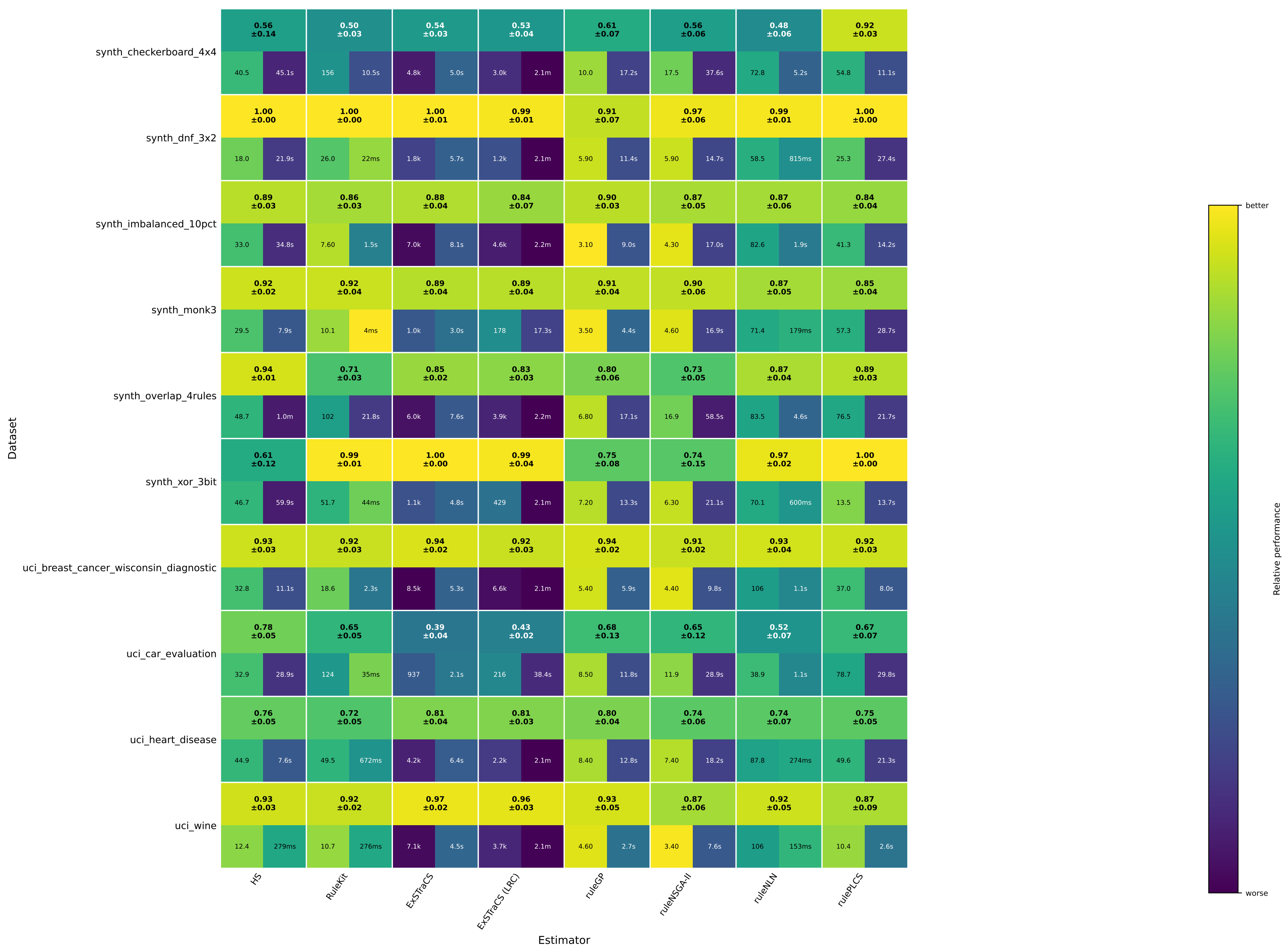
Combined benchmark heatmap: F1 (top), atoms (bottom-left), fit time (bottom-right)
