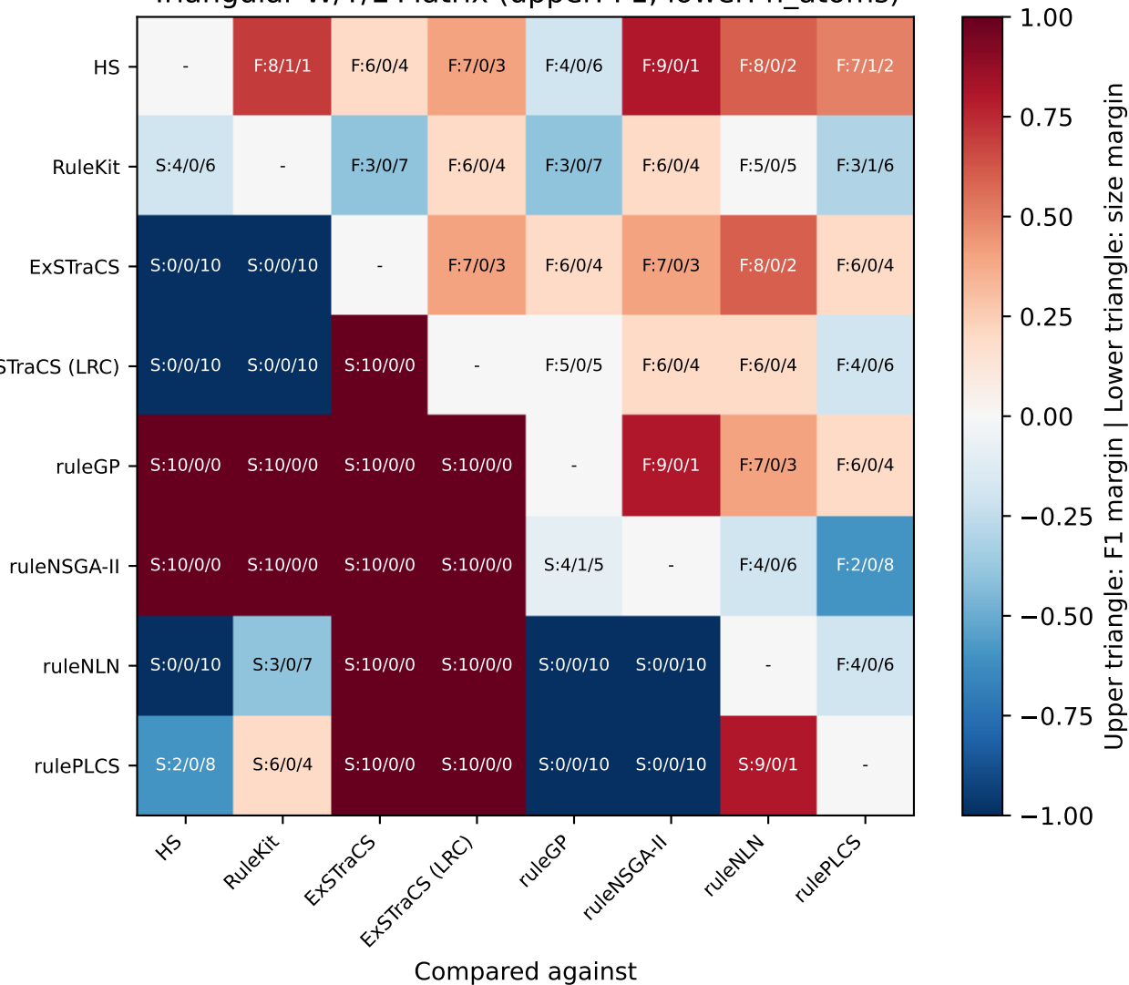
Triangular W/T/L Matrix (upper: F1, lower: n_atoms)
