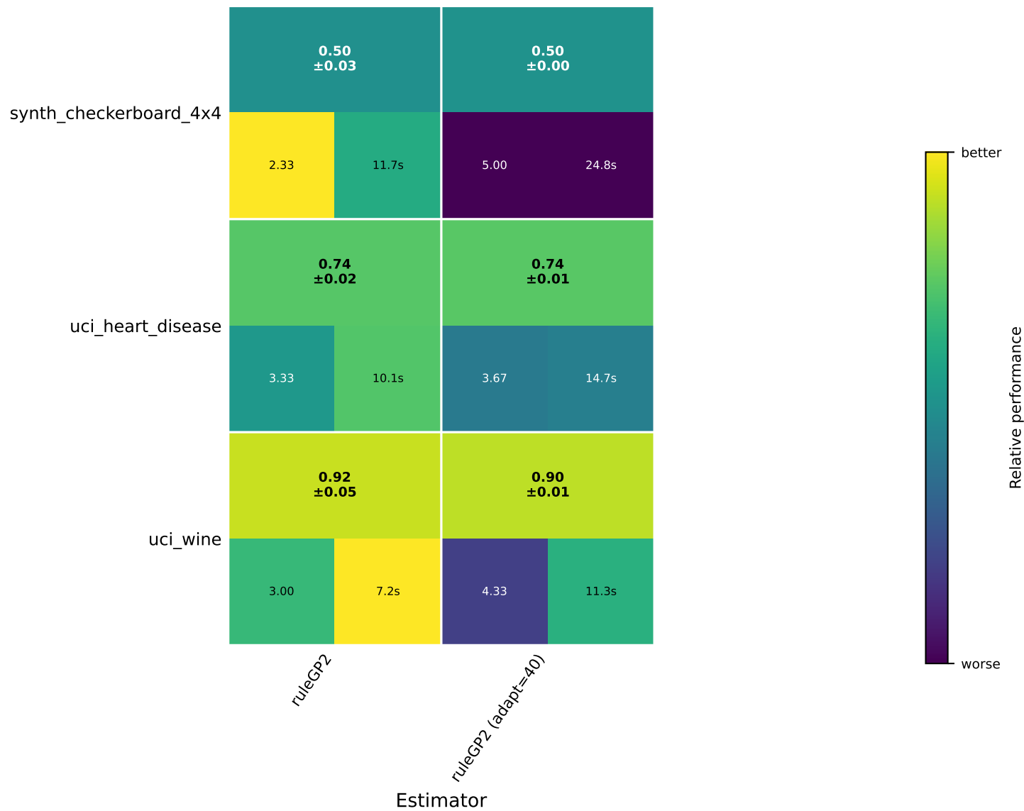
Combined benchmark heatmap: F1 (top), atoms (bottom-left), fit time (bottom-right)
