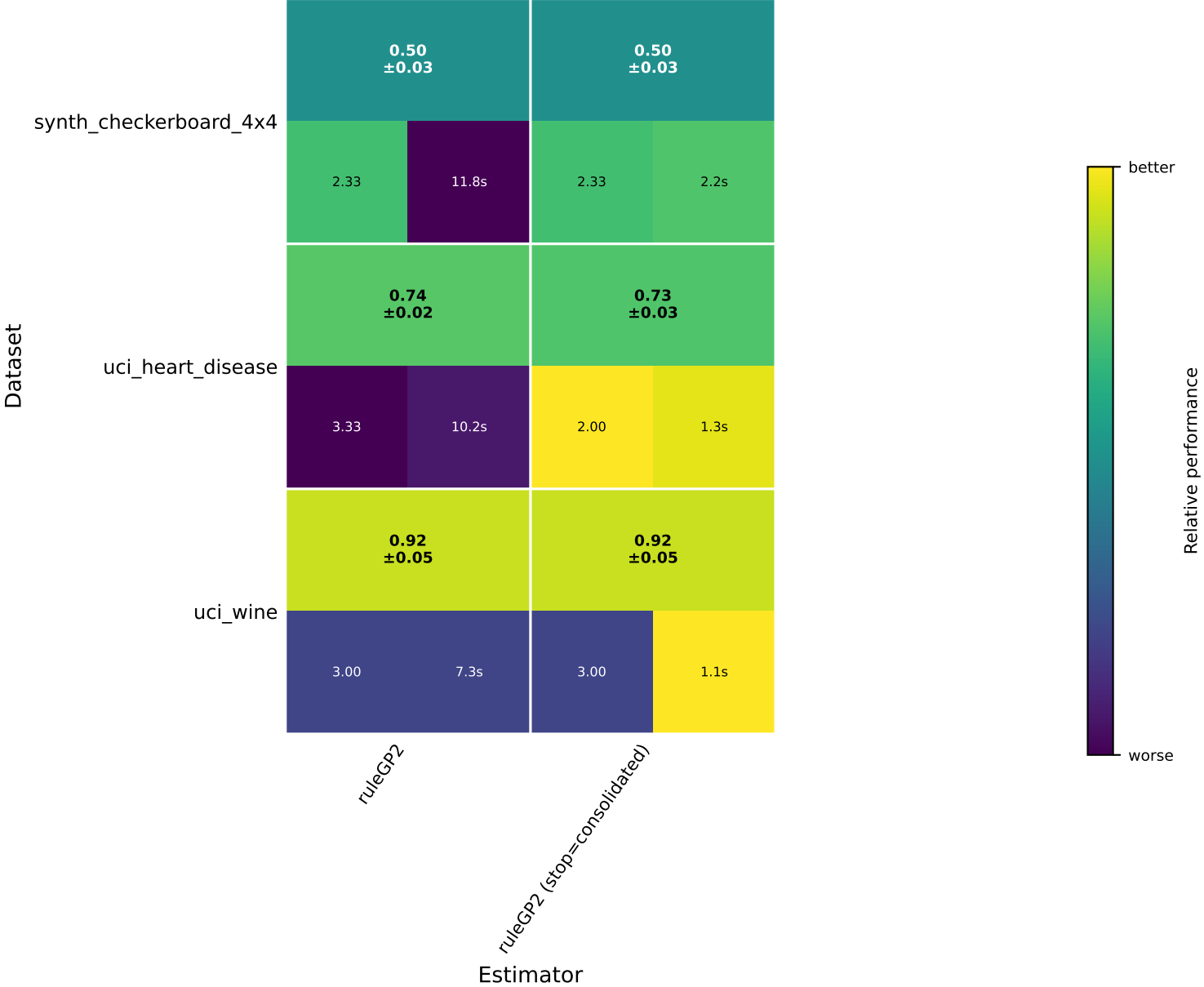
Combined benchmark heatmap: F1 (top), atoms (bottom-left), fit time (bottom-right)
