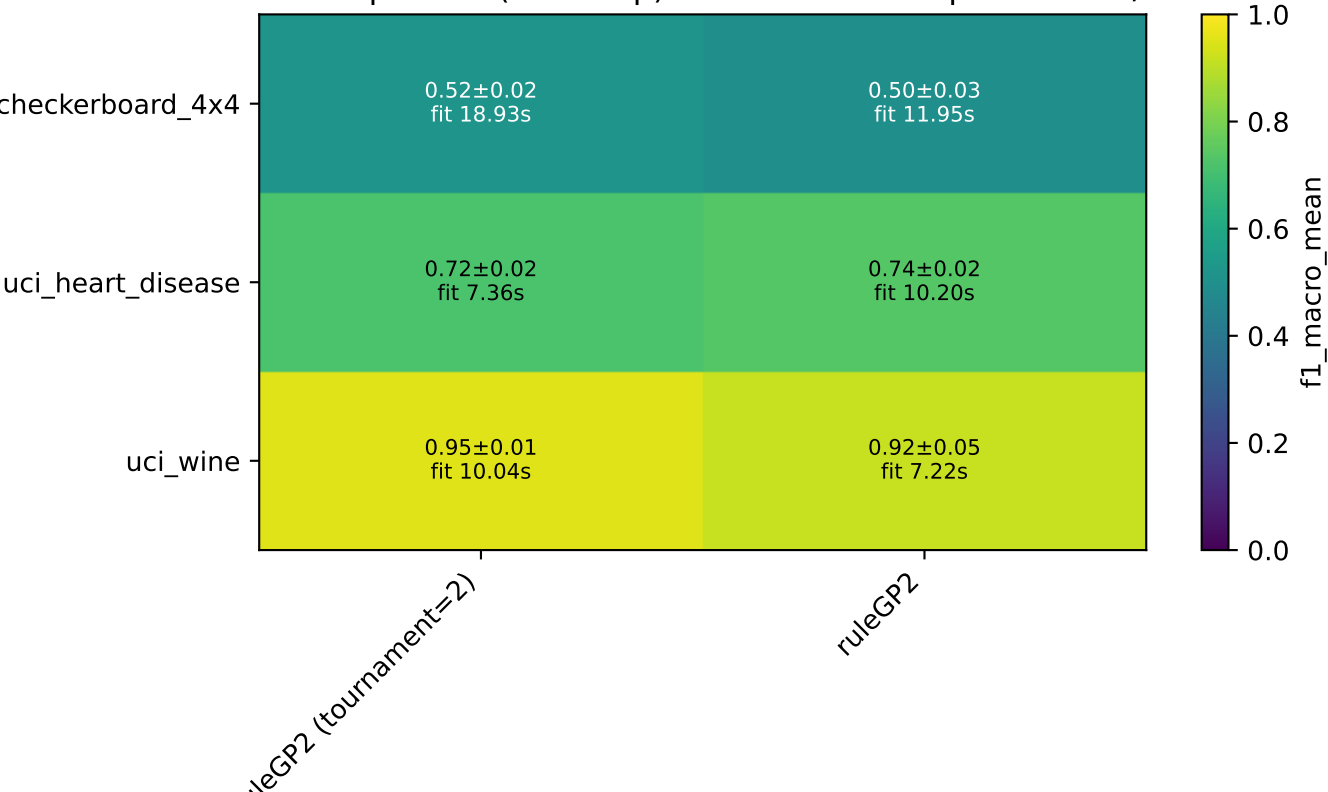
Benchmark comparison (heatmap): mean F1-macro per dataset/estimator
