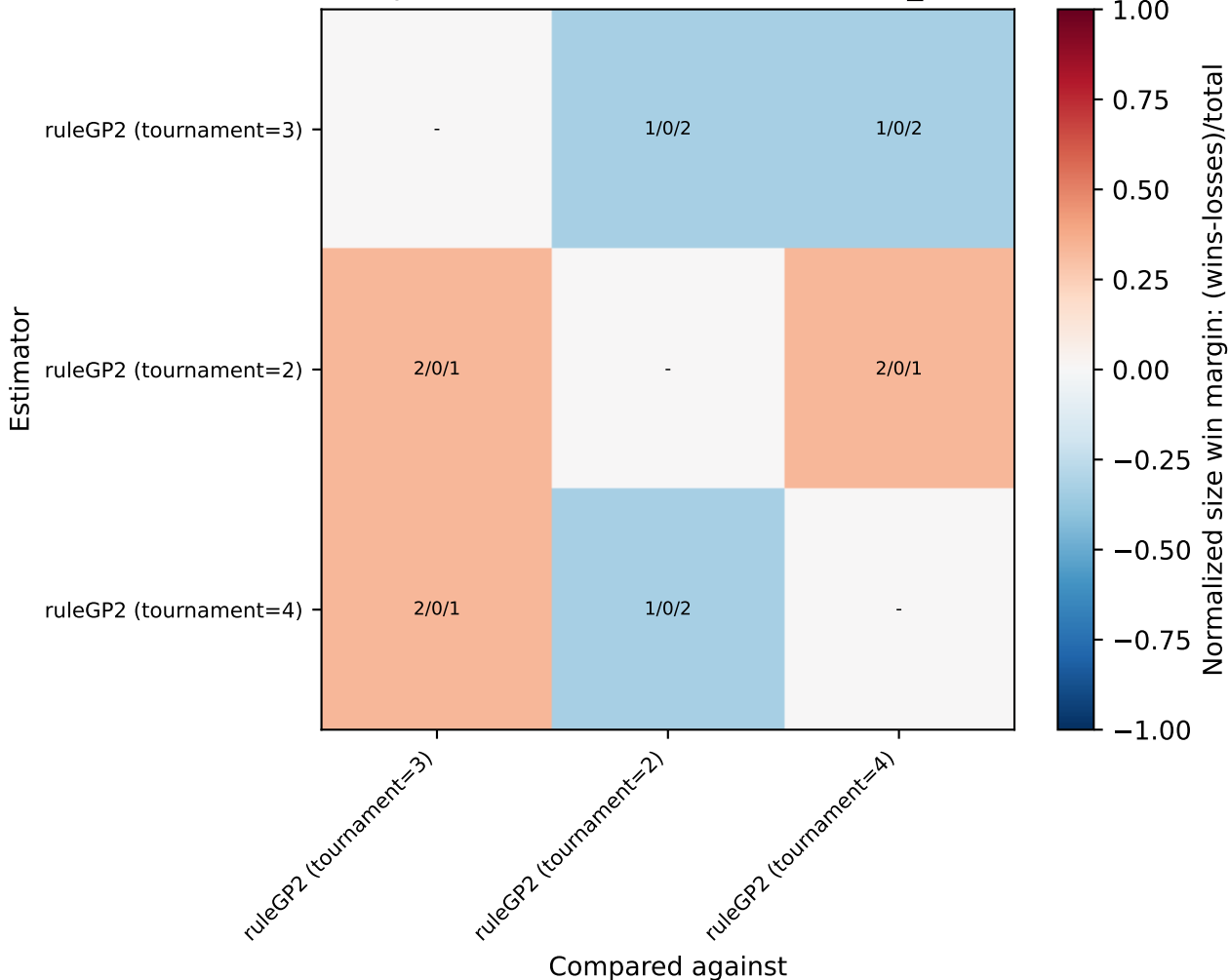
Win/Tie/Loss Matrix (pairwise over datasets, metric: n_atoms lower is better)
