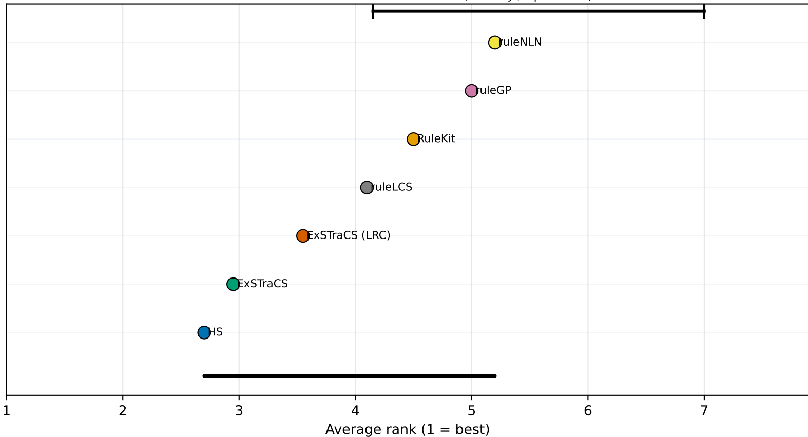
Critical Difference Diagram (F1 ranks across 10 datasets)
