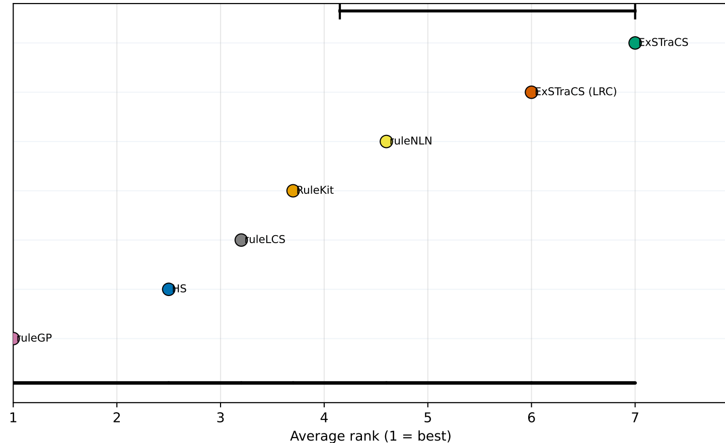
Model Complexity — atoms (10 datasets)
