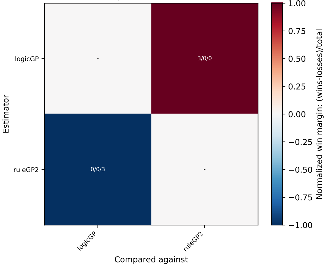
Win/Tie/Loss Matrix (pairwise over datasets, metric: F1)
