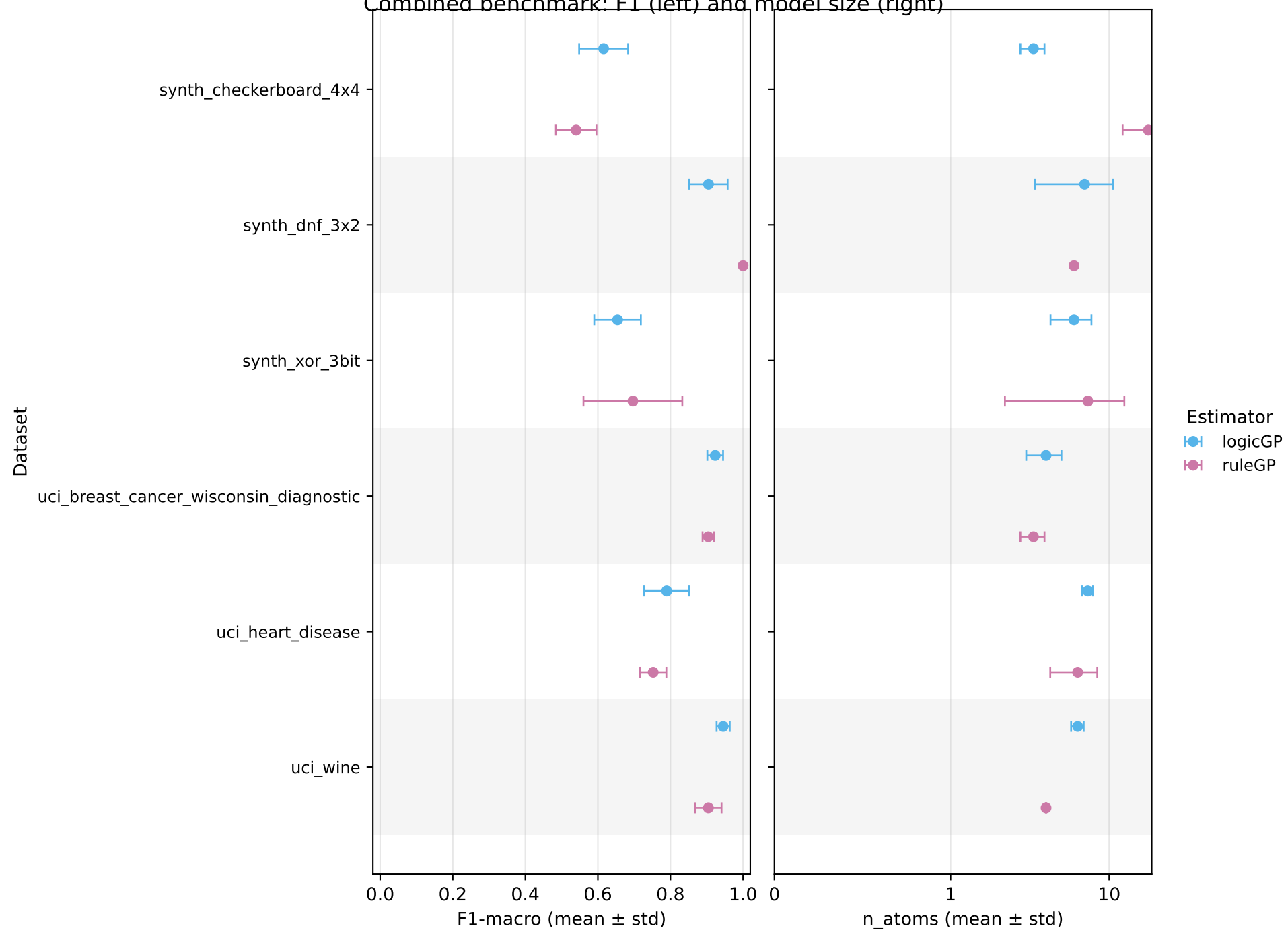
Combined benchmark: F1 (left) and model size (right)
