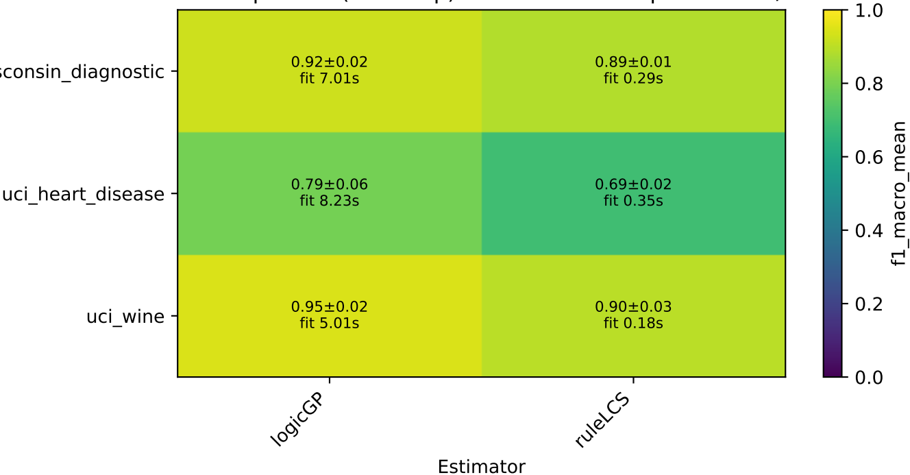
Benchmark comparison (heatmap): mean F1-macro per dataset/estimator
