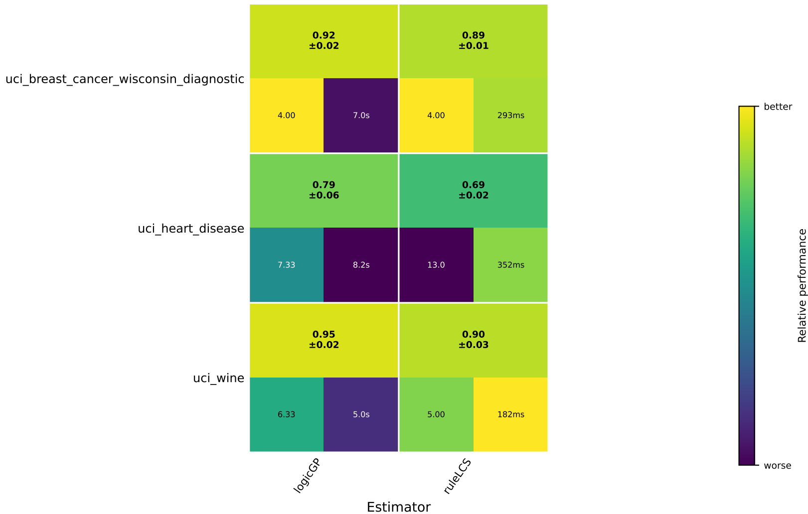
Combined benchmark heatmap: F1 (top), atoms (bottom-left), fit time (bottom-right)
